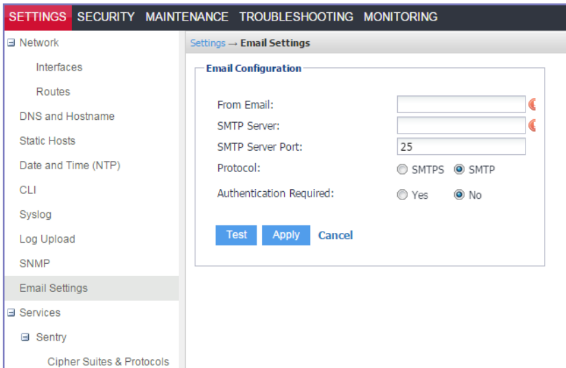
FIGURE 1. SMTP SETTINGS
