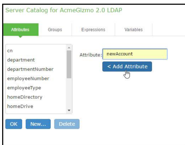
Figure 93: Server Catalog > Attributes Tab — Adding an Attribute for LDAP
