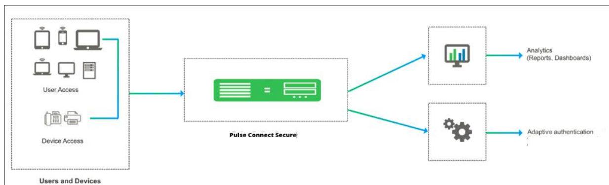
Figure 97: Behavioral Analytics
