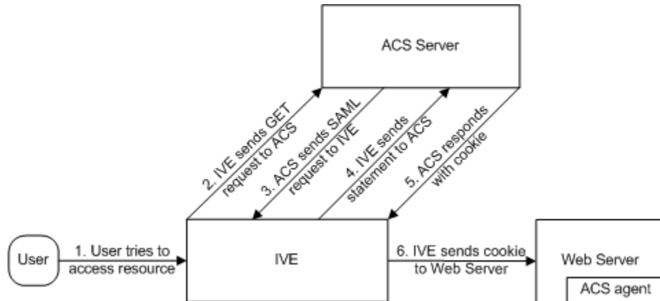
Figure 43: Artifact Profile
