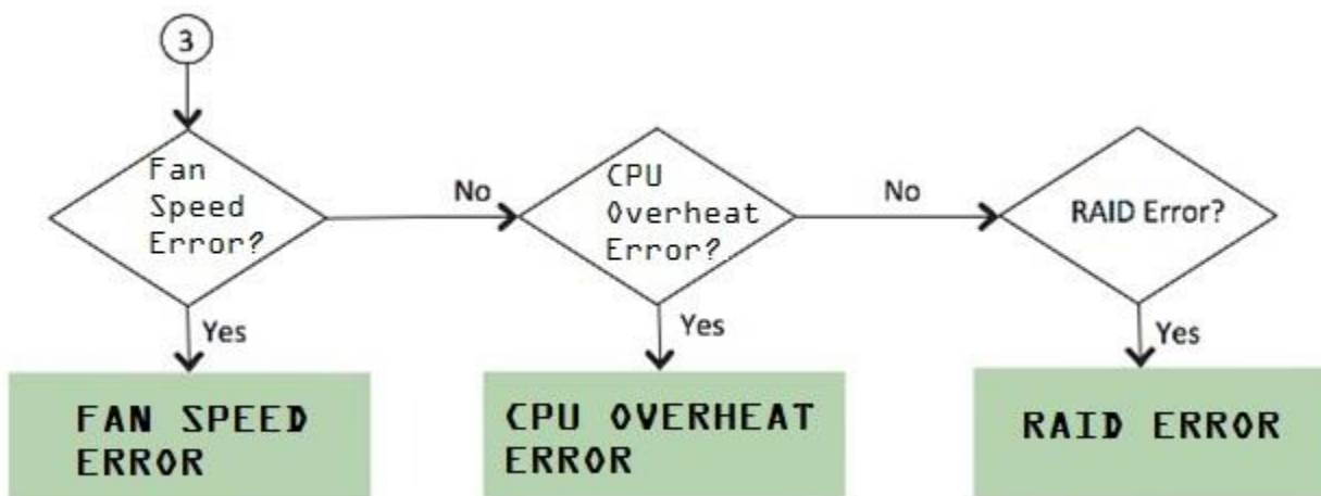
Figure 246: Error Conditions
