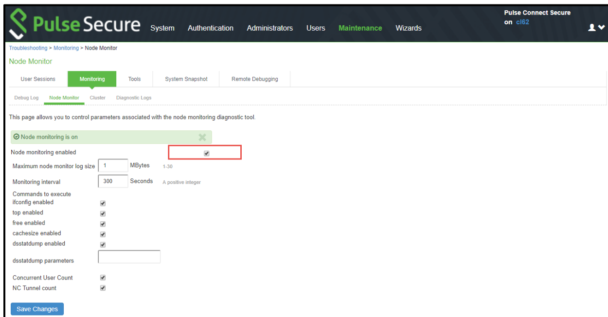
Figure 298: Troubleshooting using Node Monitor
