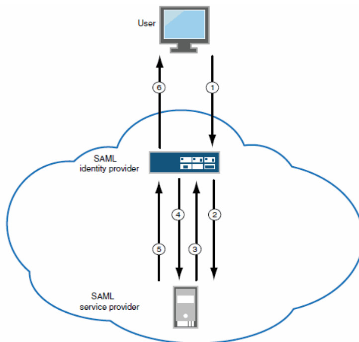
Figure 26: Connect Secure as a SAML Identity Provider (Gateway Mode) – User/Browser Action Not Required
