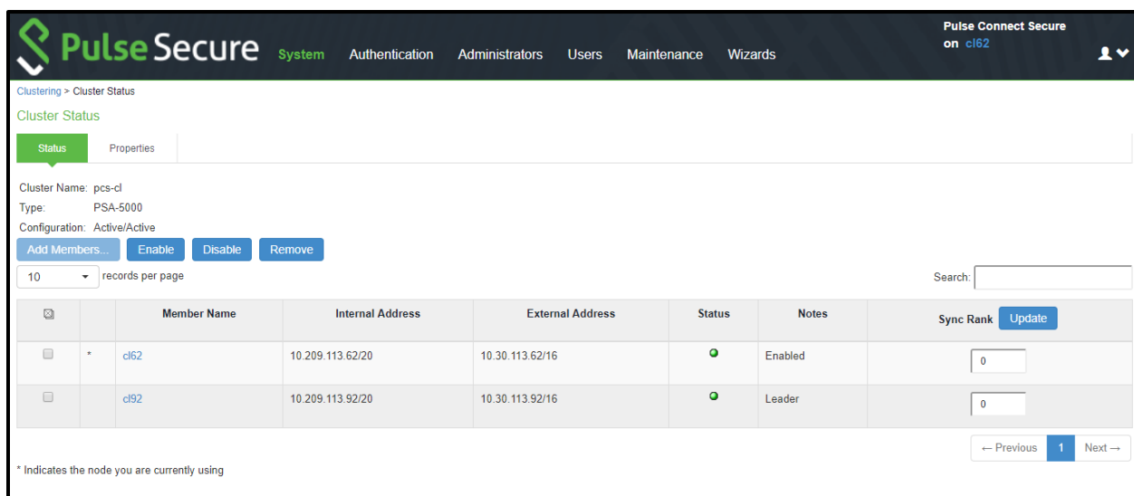
Figure 278: Clustering Page –Status
