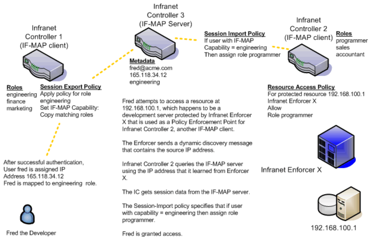
Figure 4: Session-Import and Session-Export Policies
