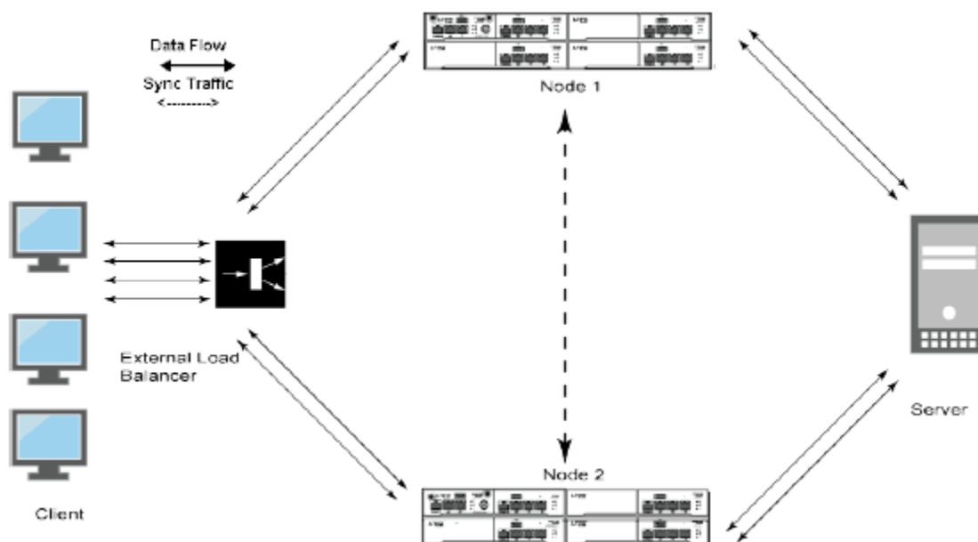
Figure 271: Active/Active Clustering
