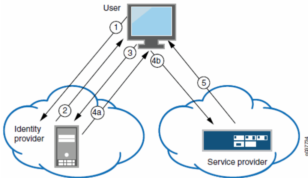
Figure 24: Connect Secure as a SAML Service Provider in an Identity-Provider-Initiated SSO Scenario
