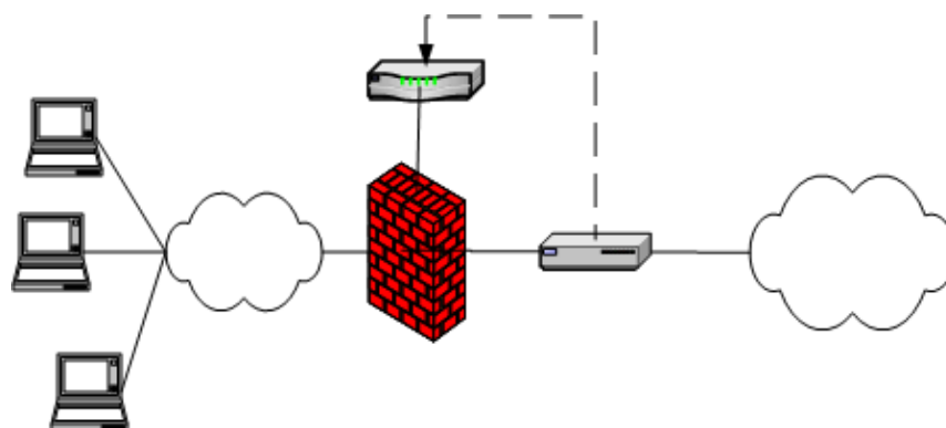
Figure 305: Pulse Connect Secure and IDP Topology Scenario 1
