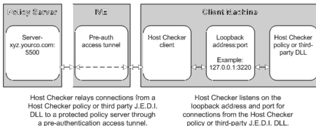
Figure 113: Host Checker Creates a Tunnel from a Client to a Policy Server Behind Connect Secure
