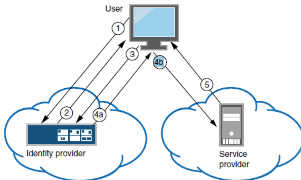
Figure 29: Connect Secure as a SAML Identity Provider (Peer Mode) in an Identity-Provider-Initiated SSO Scenario
