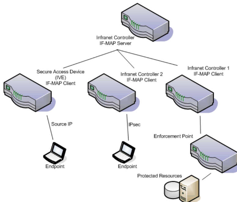
Figure 3: IF-MAP Federated Network Topology
