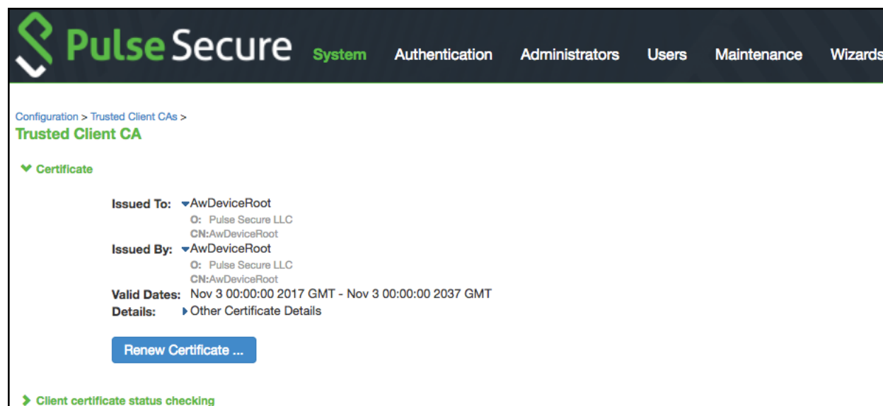
Figure 57: Trusted Client CA Configuration for AirWatch
