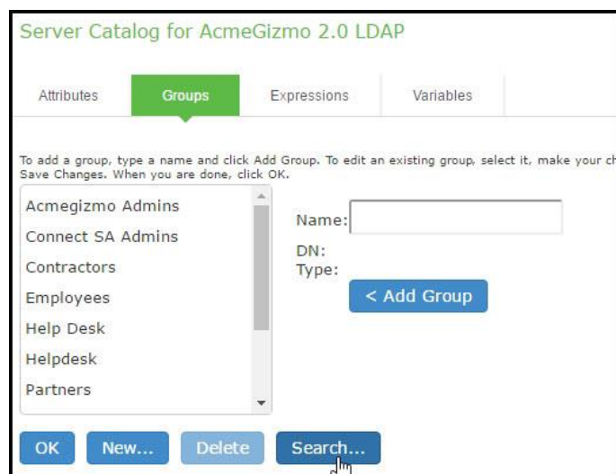
Figure 94: Server Catalog > Groups Tab — Adding LDAP Groups
