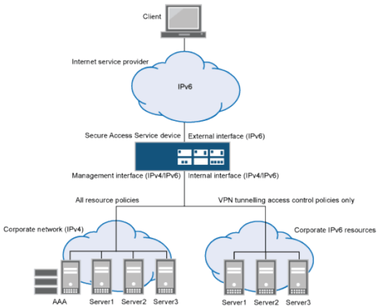
Figure 166: Dual Stack Endpoint Access Over ISP IPv6 Network
