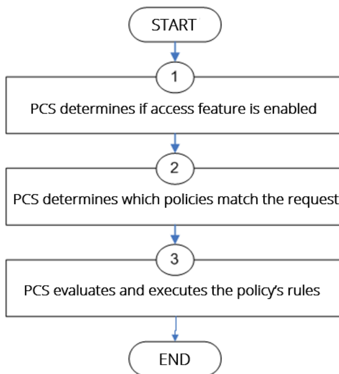
Figure 8: Resource Policy Evaluation Steps
