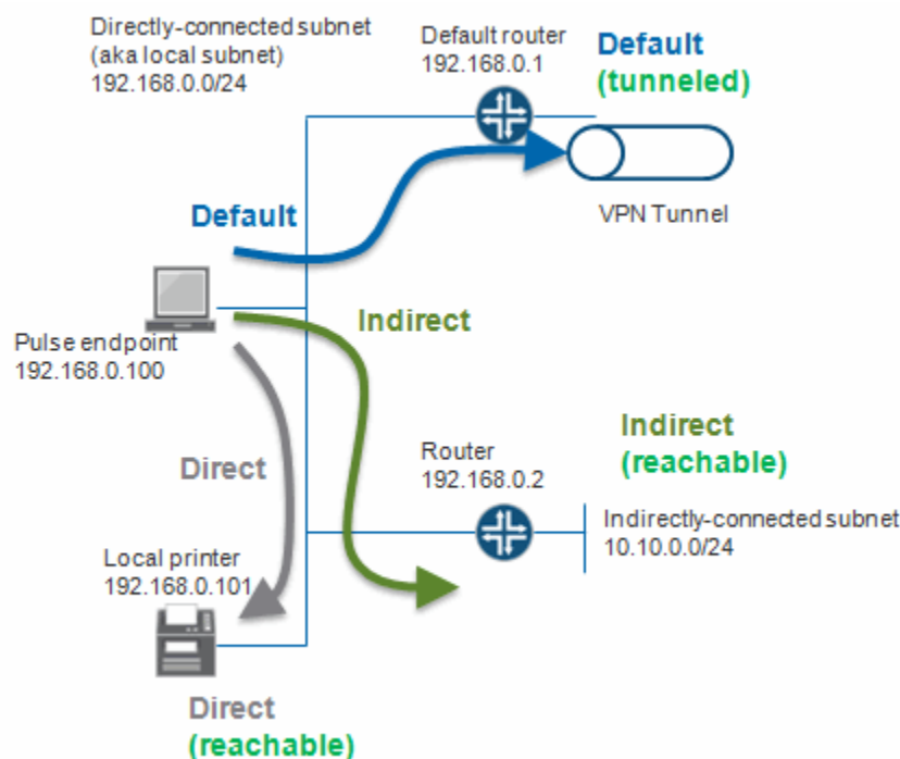
Figure 139: Endpoint Route Precedence Example
