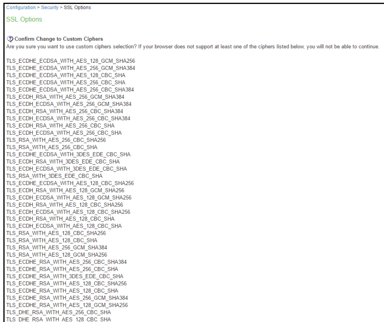
Figure 205: Confirming Custom Ciphers
