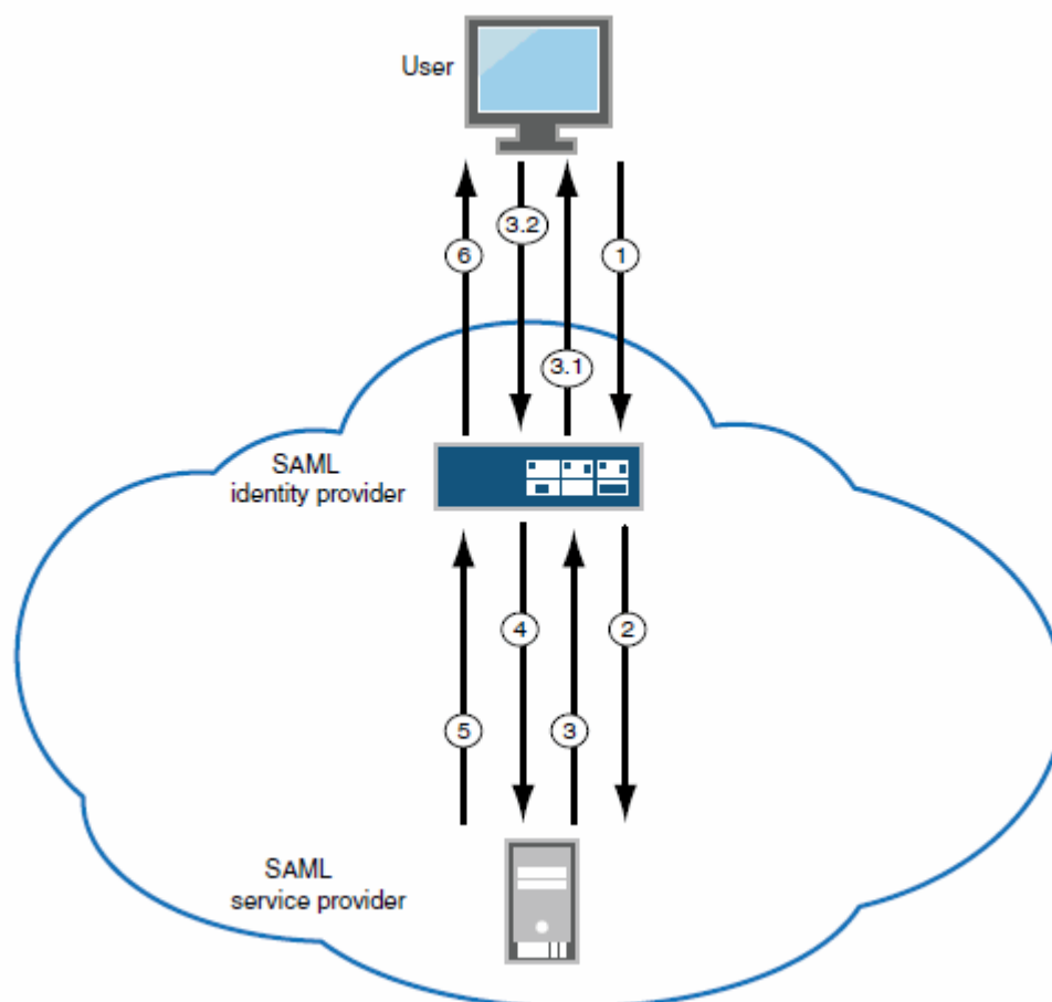
Figure 27: Connect Secure as a SAML Identity Provider (Gateway Mode) – User/Browser Action Required
