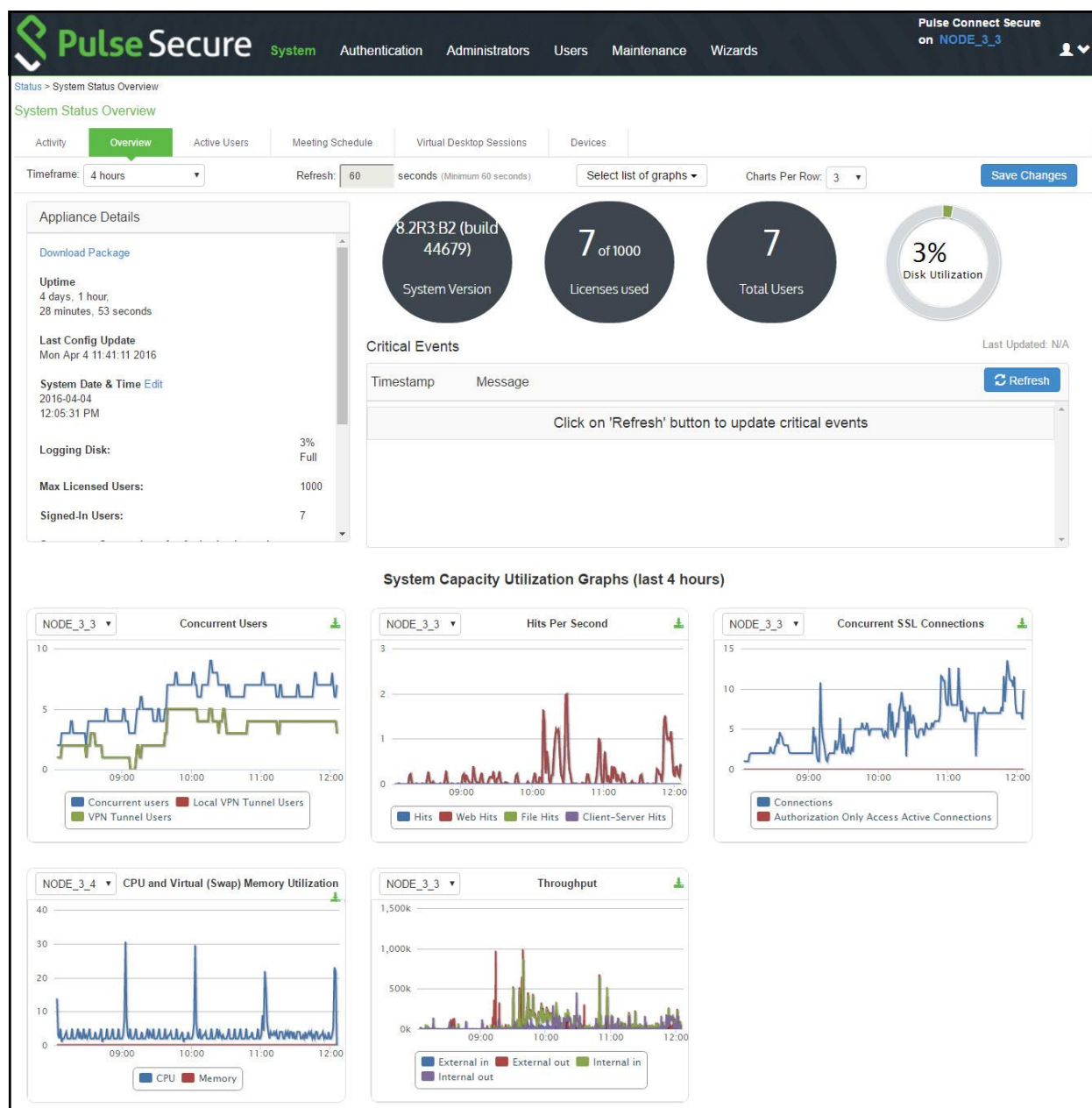
Figure 240: System Status Page – Pulse Connect Secure
