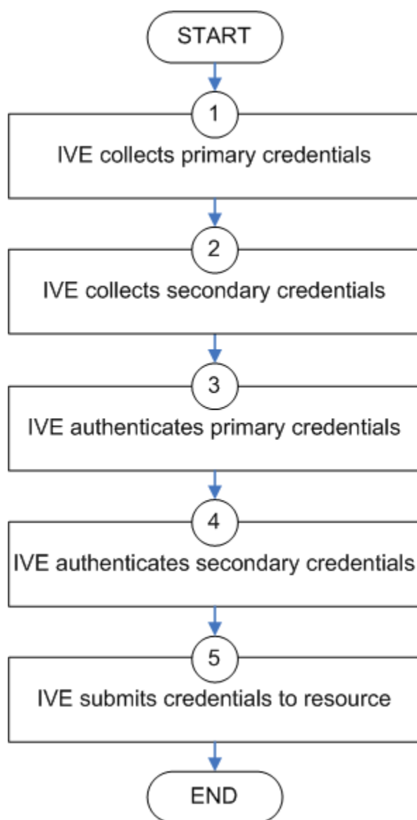
Figure 96: Collecting and Submitting Credentials from Multiple Servers
