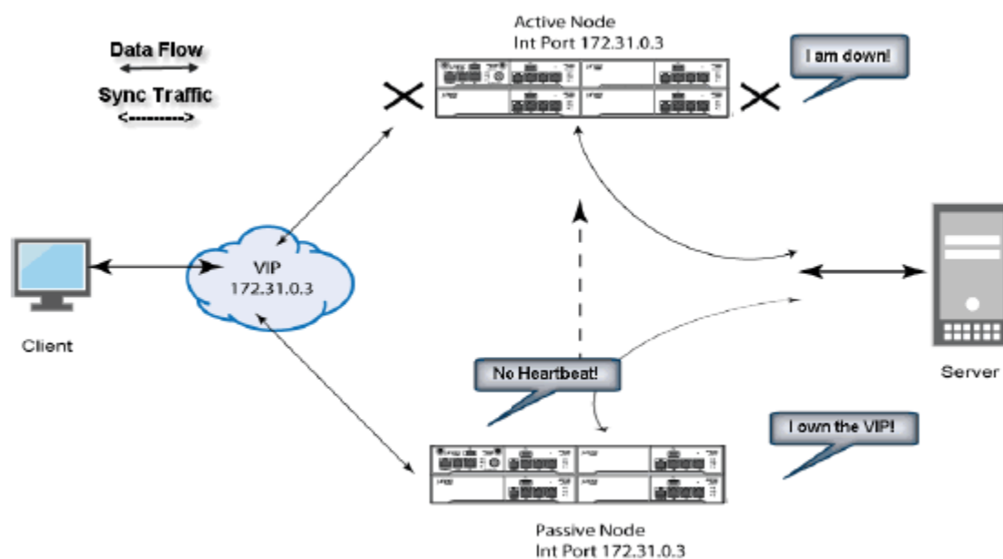
Figure 279: Active/Passive Clustering
