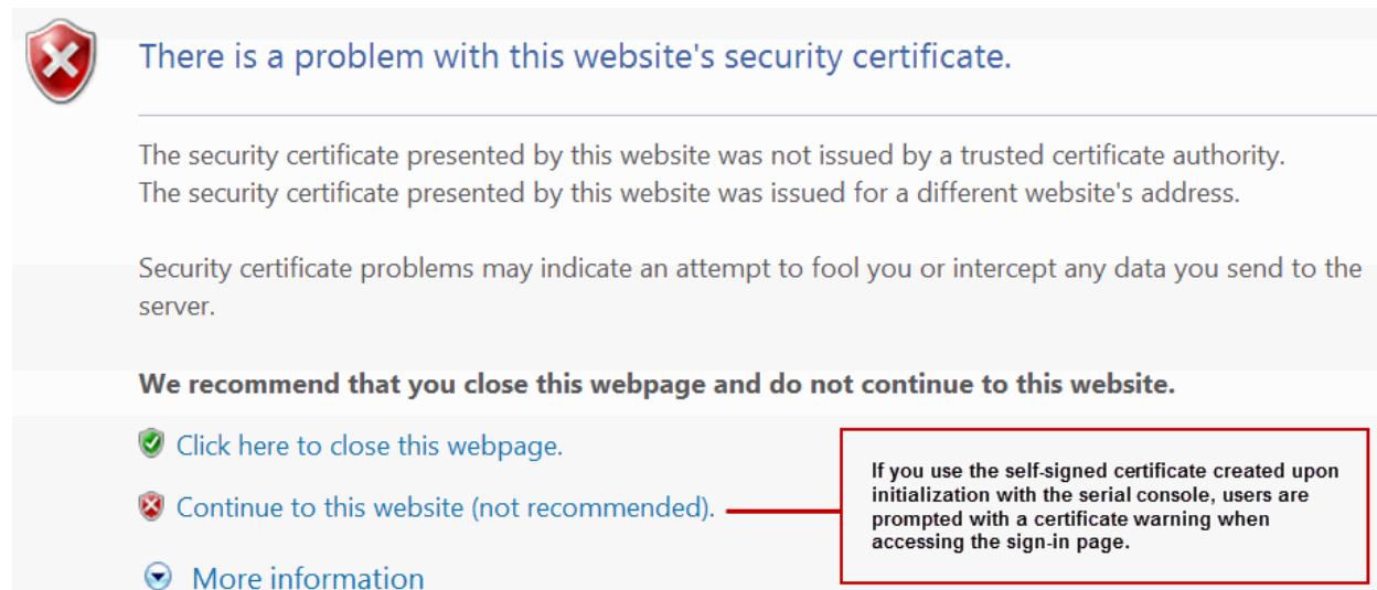
Figure 184: Security Alert When the Device Certificate Is Not Issued by a Trusted CA
