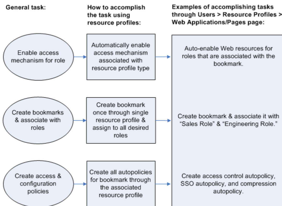
Figure 7: Using Resource Profiles to Configure Resources
