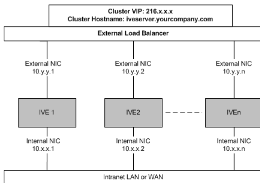
Figure 287: Active/Active Configuration
