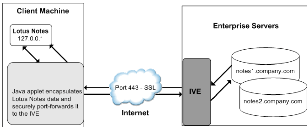
Figure 123: Java Secure Application Manager and Enhanced Lotus Notes Support
