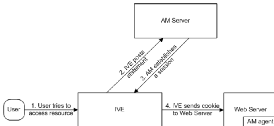
Figure 45: Access Control Policies
