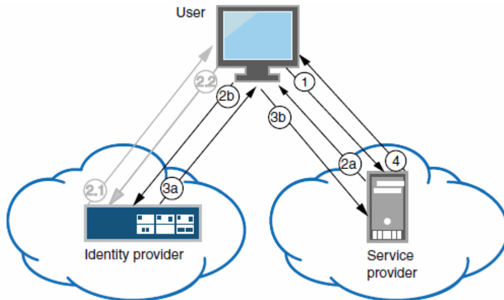
Figure 30: Connect Secure as a SAML Identity Provider (Peer Mode) in a Service-Provider-Initiated SSO Scenario
