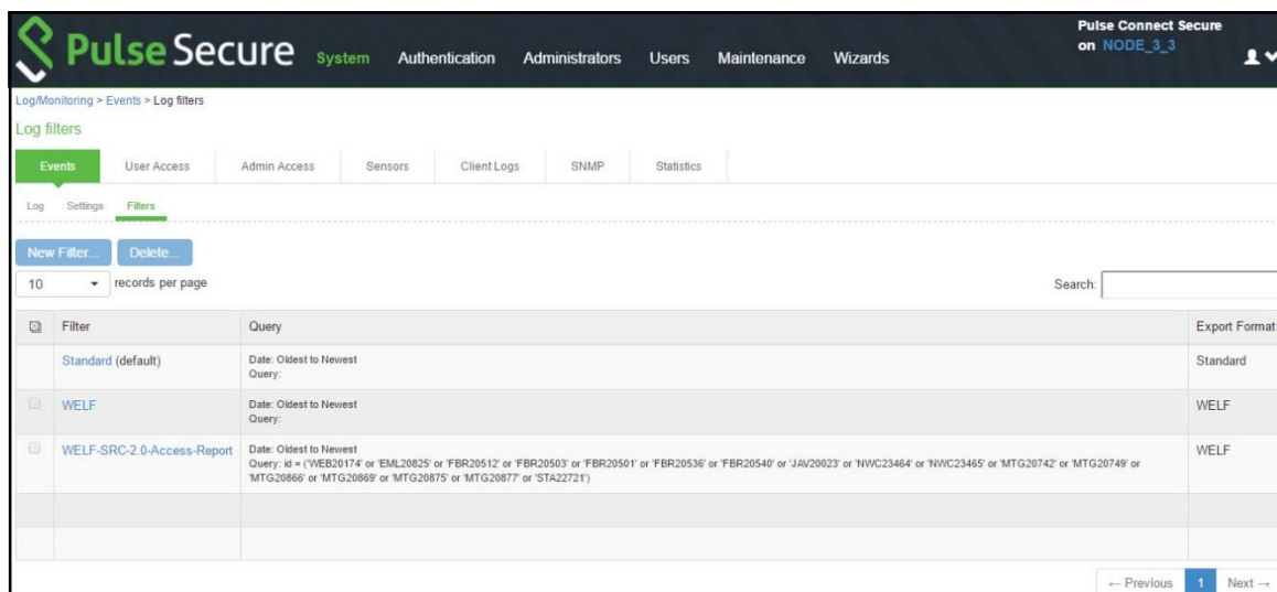
Figure 249: Log Filters Page – Pulse Connect Secure
