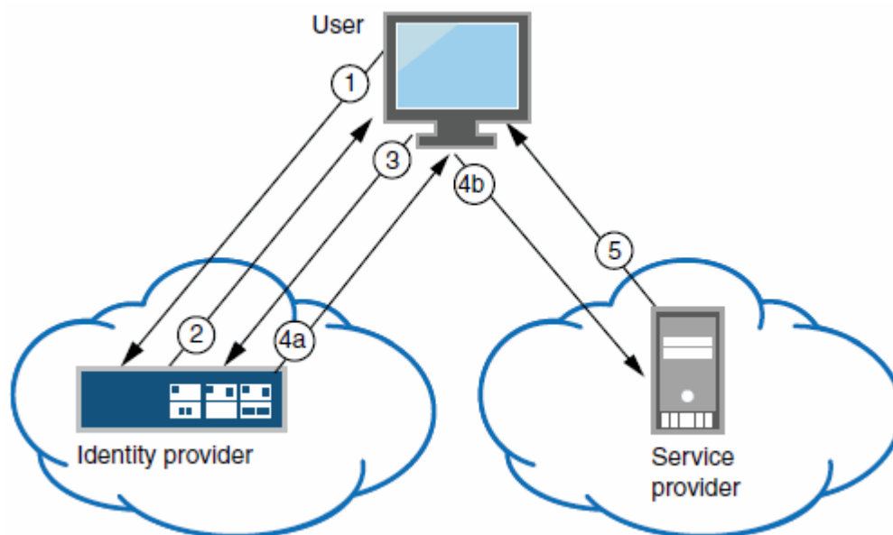
Figure 31: Connect Secure as a SAML Identity Provider (Peer Mode) in an Identity-Provider-Initiated SSO Scenario
