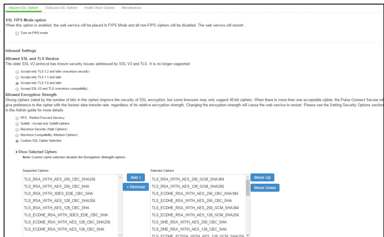
Figure 202: Supported Ciphers and Selected Ciphers Panels
