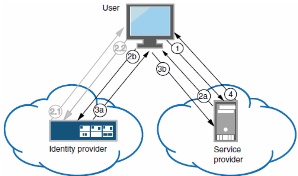
Figure 28: Connect Secure as a SAML Identity Provider (Peer Mode) in a Service-Provider-Initiated SSO Scenario
