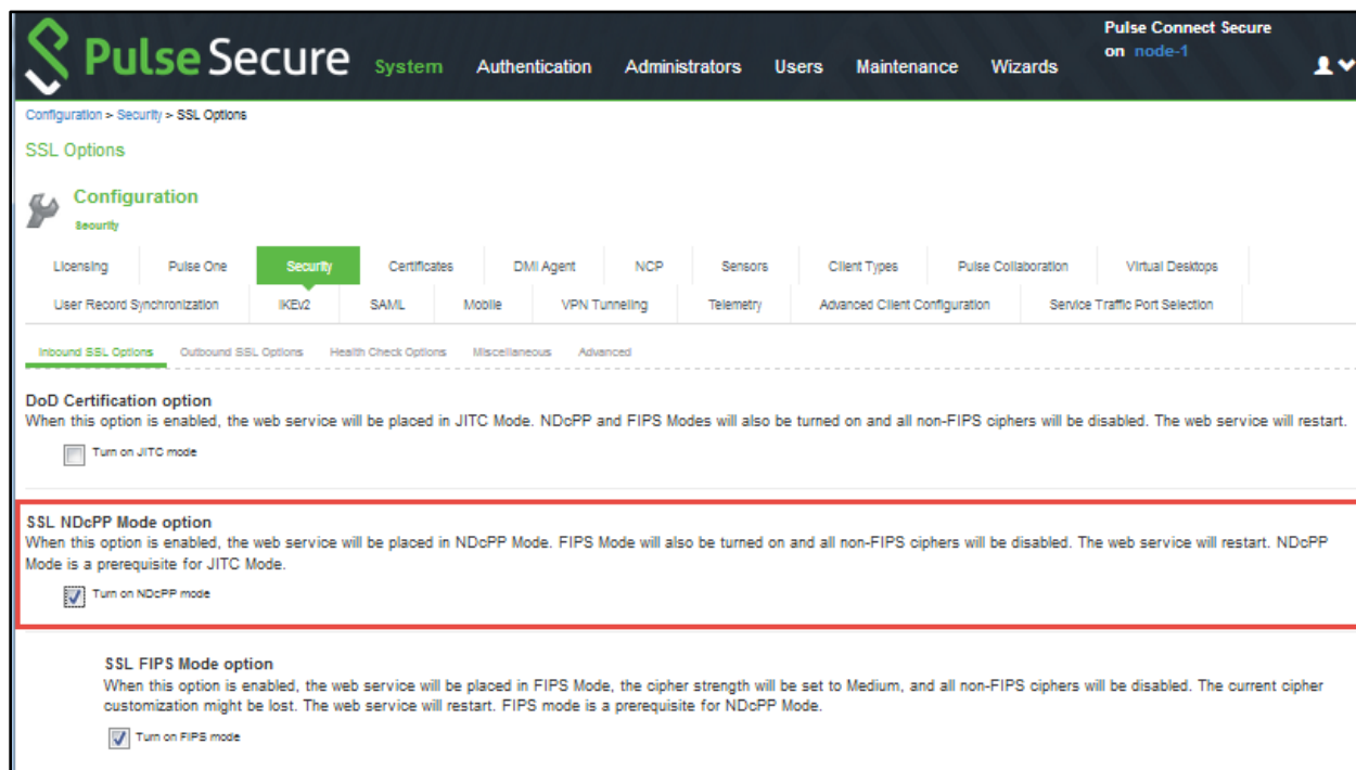
Figure 173: SSL NDcPP Mode Option
