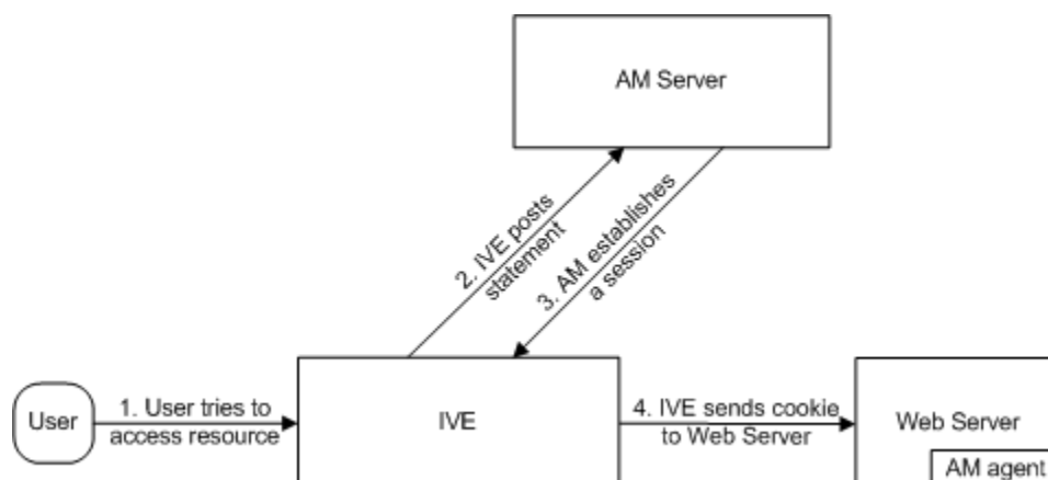
Figure 44: POST Profile
