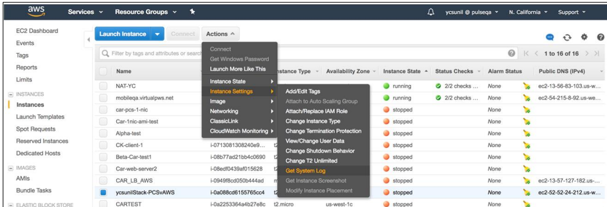
Figure 47: Boot Diagnostics
