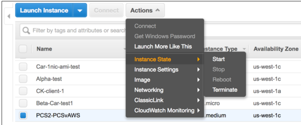
Figure 45: System Operations
