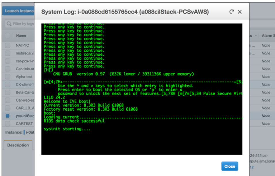
Figure 48: System Logs
