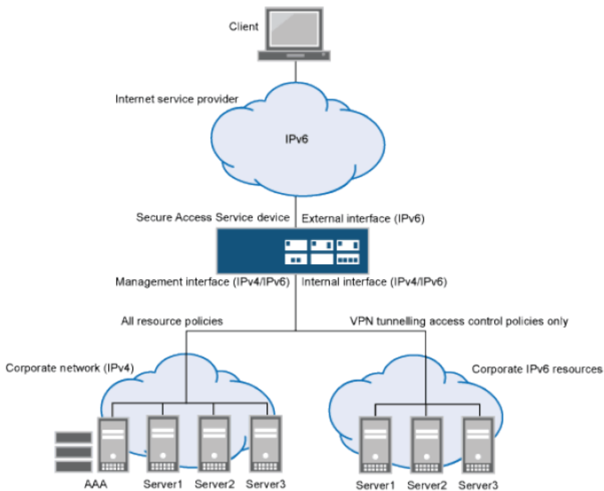
Figure 167: Dual Stack Endpoint Access Over ISP IPv6 Network
