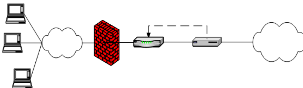
Figure 307: Pulse Connect Secure and IDP Topology Scenario 2
