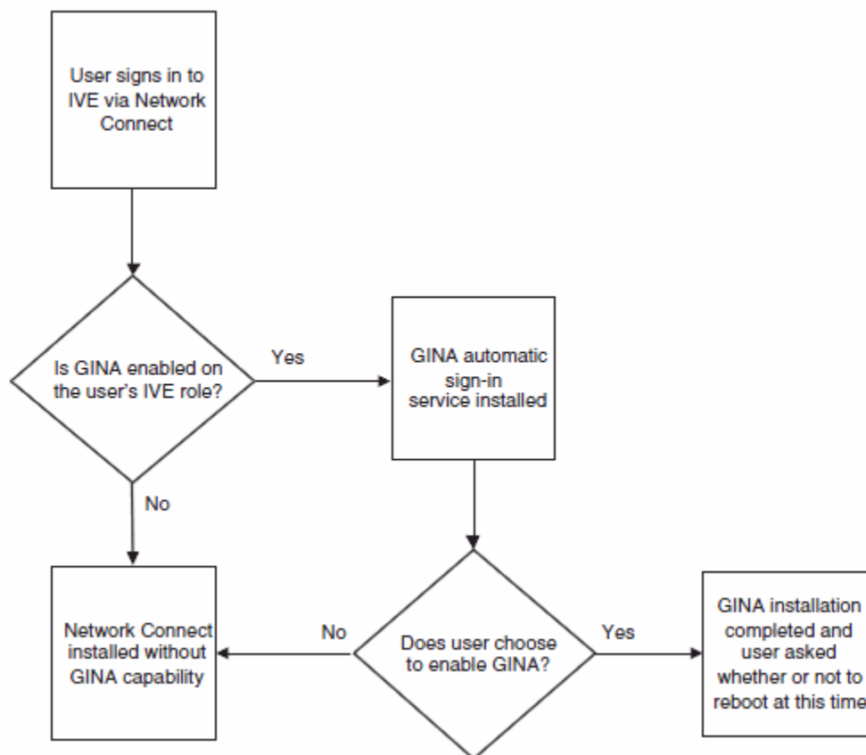
Figure 134: GINA Installation Process
