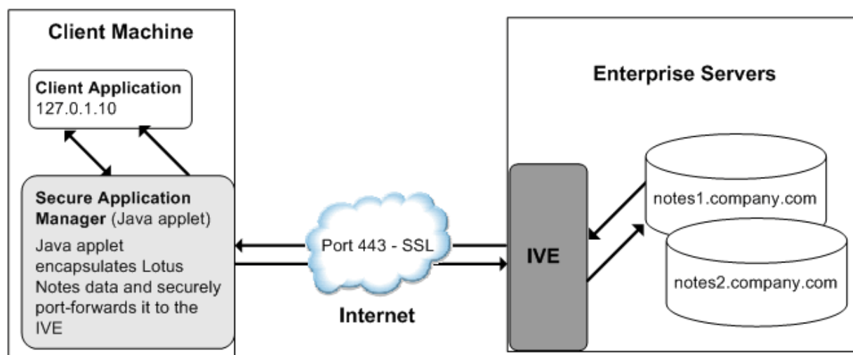
Figure 122: Java Secure Application Manager
