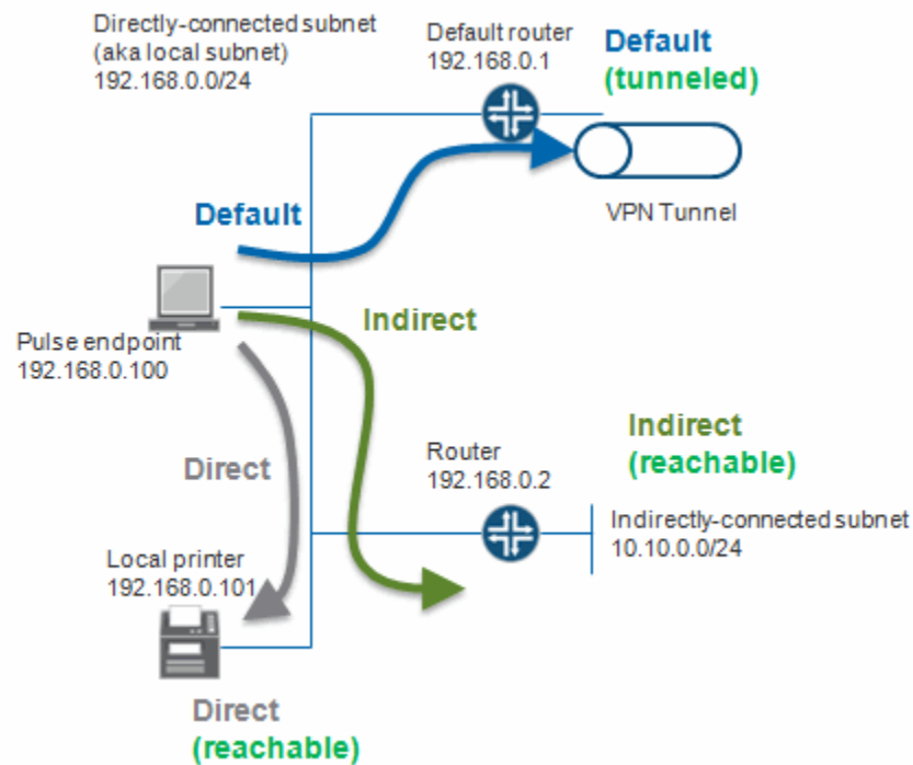
Figure 140: Endpoint Route Precedence Example
