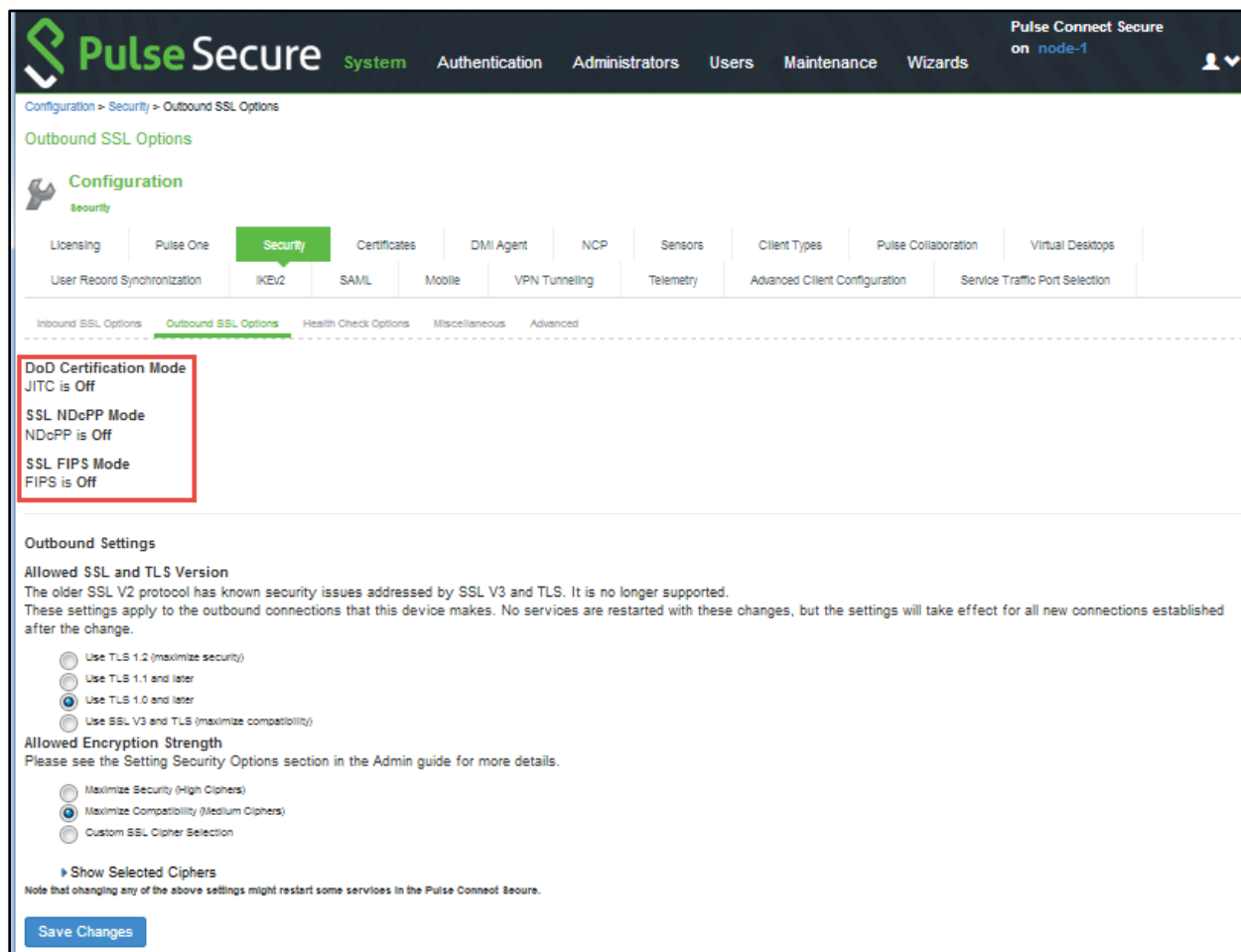
Figure 177: NDcPP Outbound Settings Page
