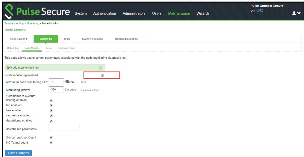
Figure 299: Troubleshooting using Node Monitor
