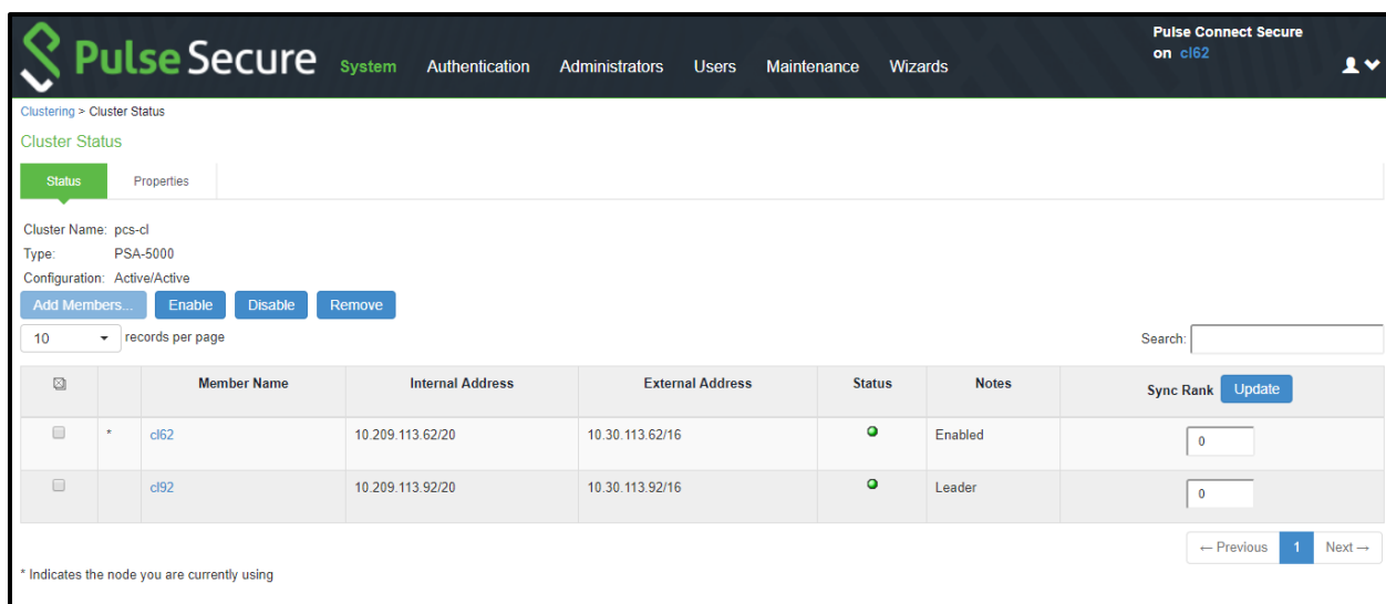
Figure 279: Clustering Page –Status
