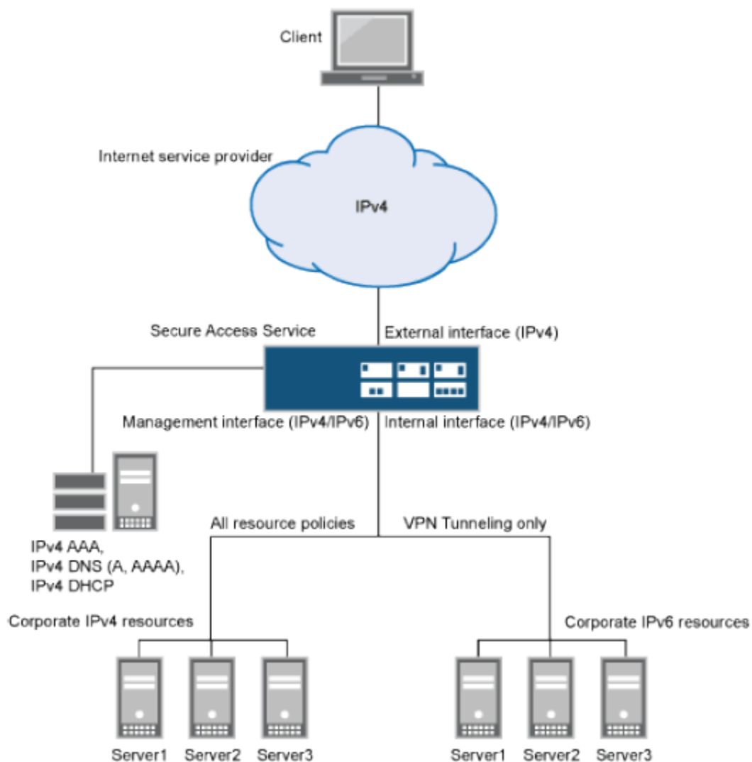
Figure 166: Dual Stack Endpoint Access Over ISP IPv4 Network
