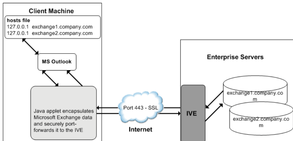
Figure 123: Java Secure Application Manager and Enhanced MS Exchange Support
