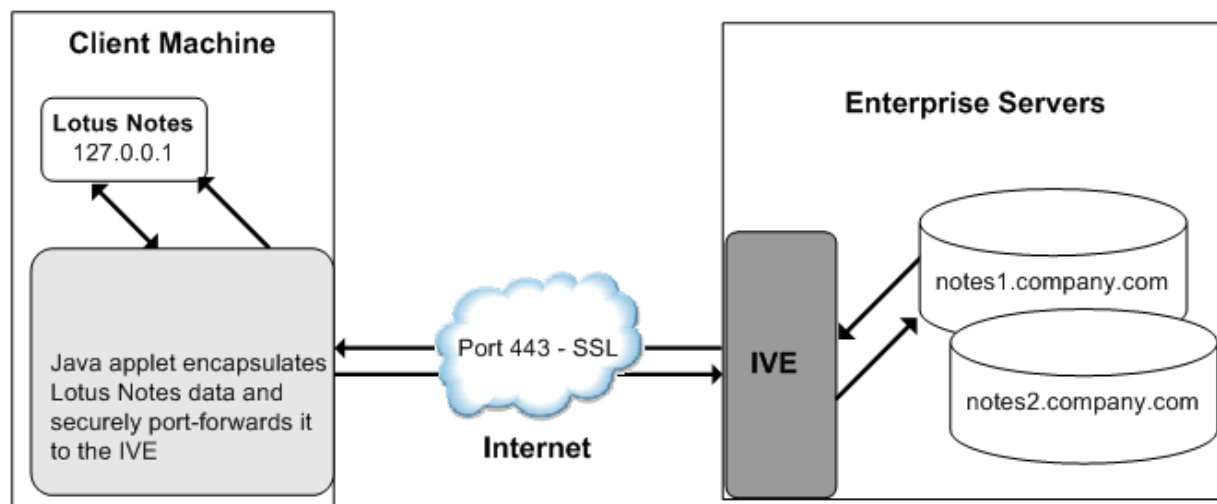
Figure 124: Java Secure Application Manager and Enhanced Lotus Notes Support
