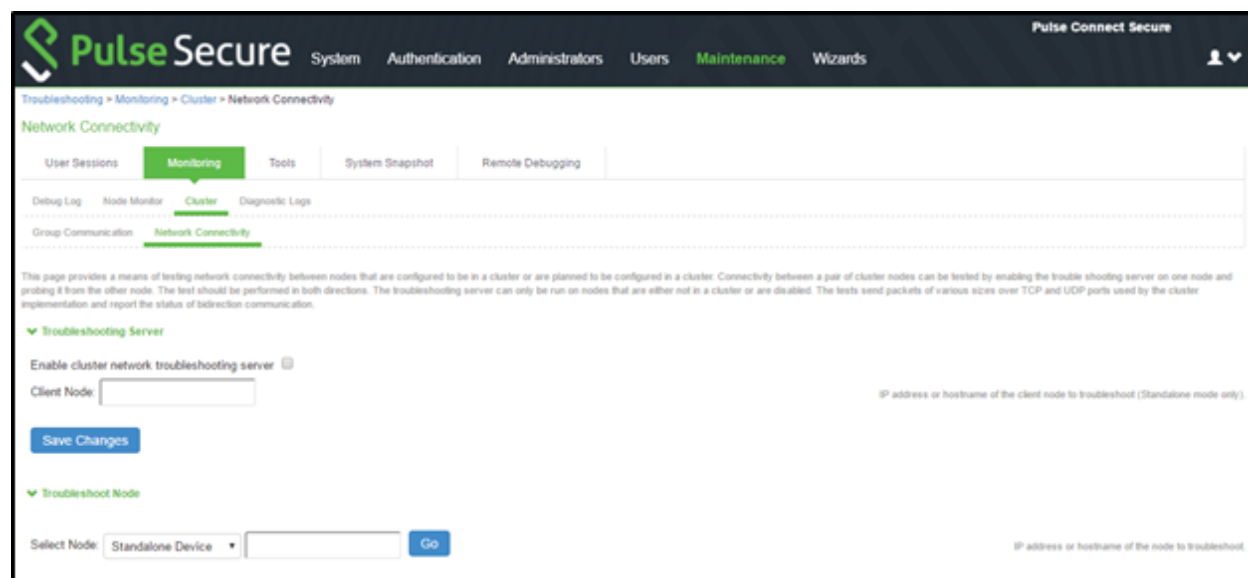
Figure 300: Troubleshooting using Network Connectivity
