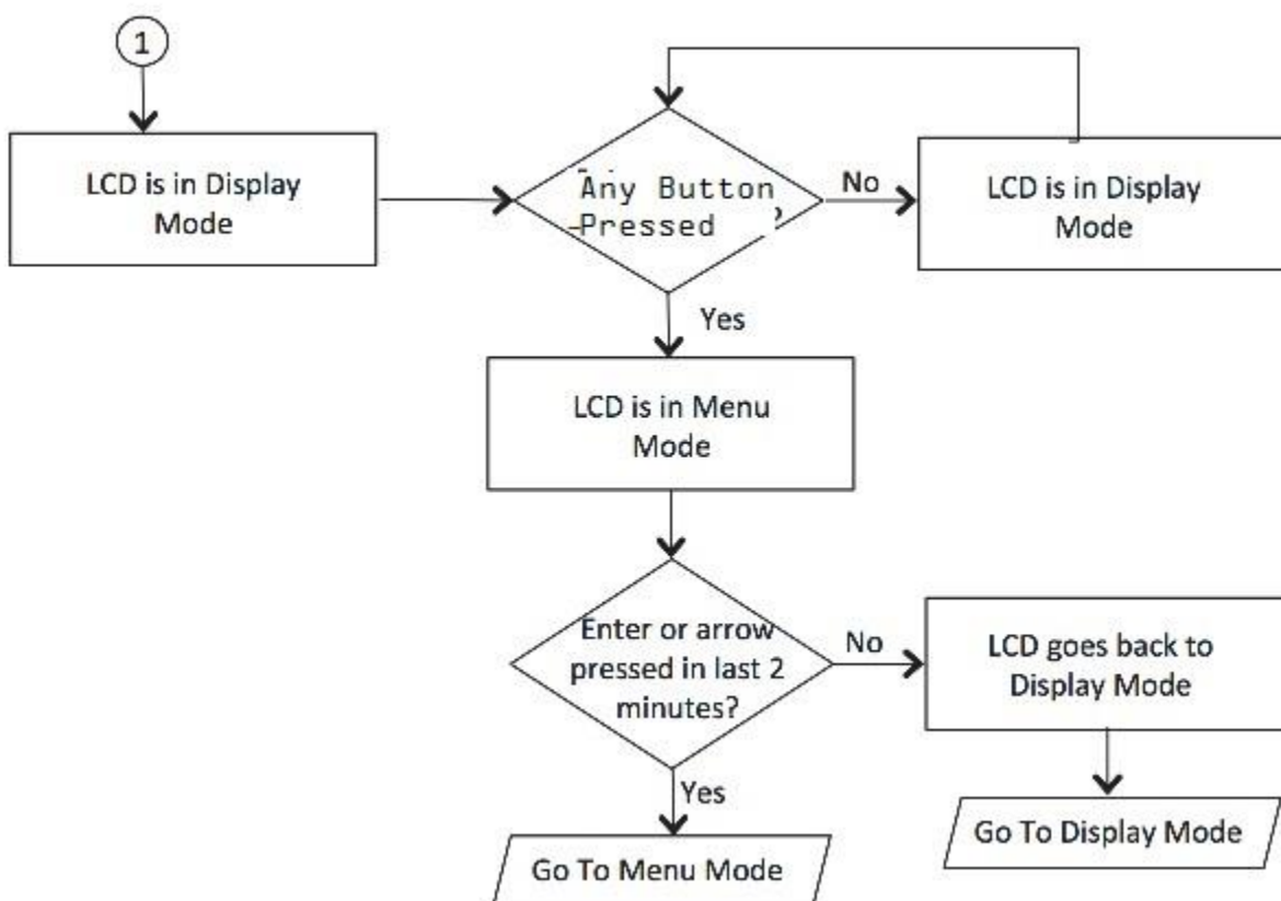
Figure 245: Two Modes Supported by the LCD
