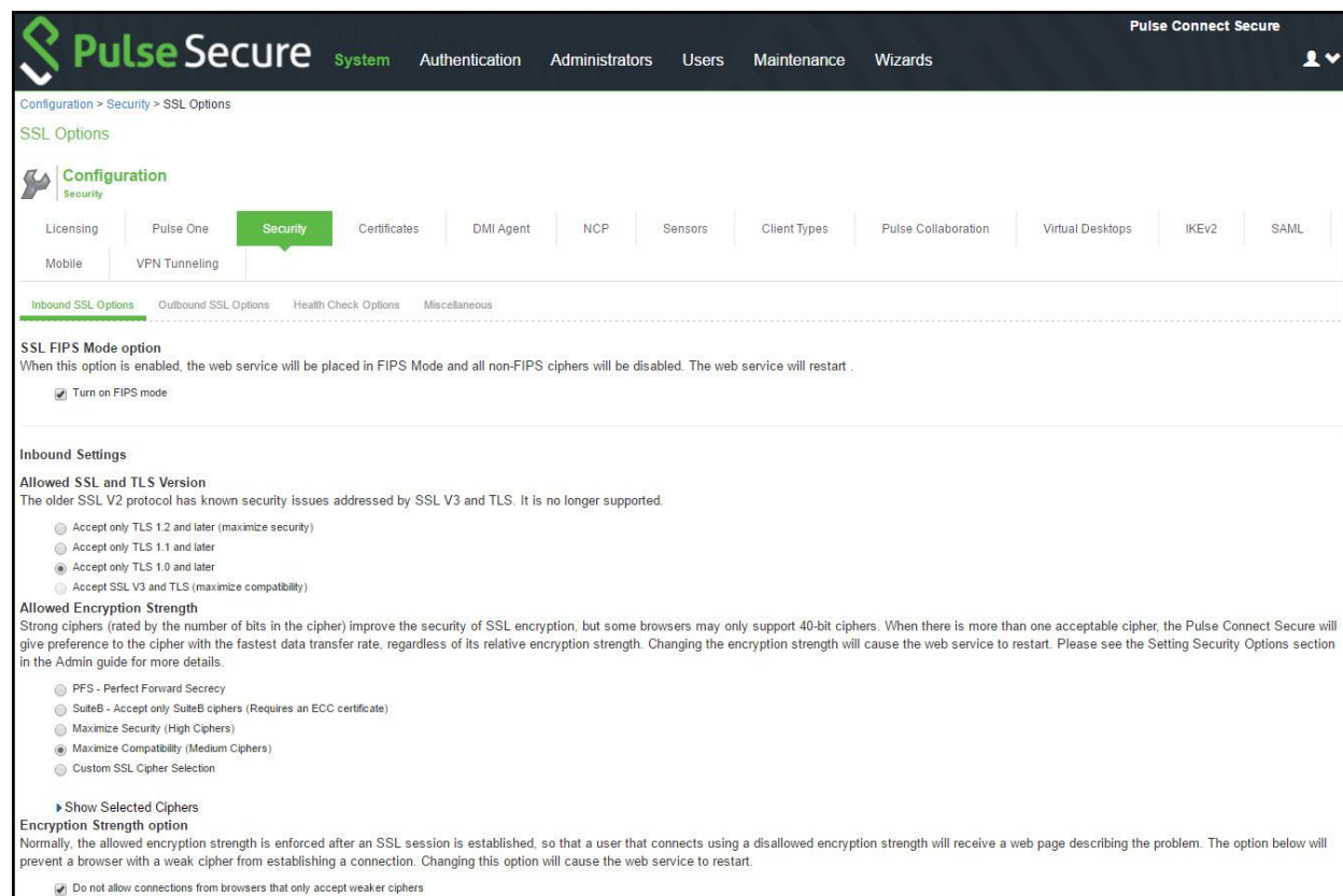
Figure 340: Enabling FIPS Level 1 Support
