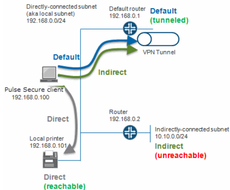
Figure 141: Tunnel Routes with Local Subnet Access Example
