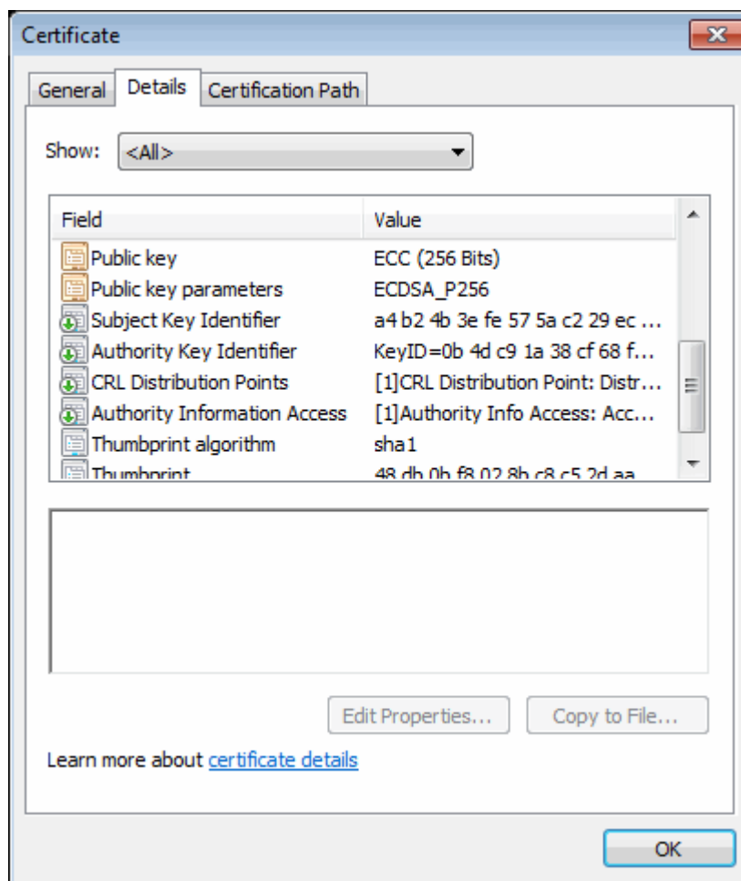
Figure 210: Certificate Public Key
