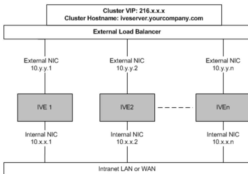
Figure 296: Active/Active Configuration
