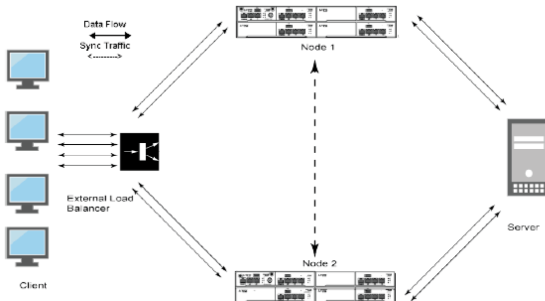
Figure 280: Active/Active Clustering
