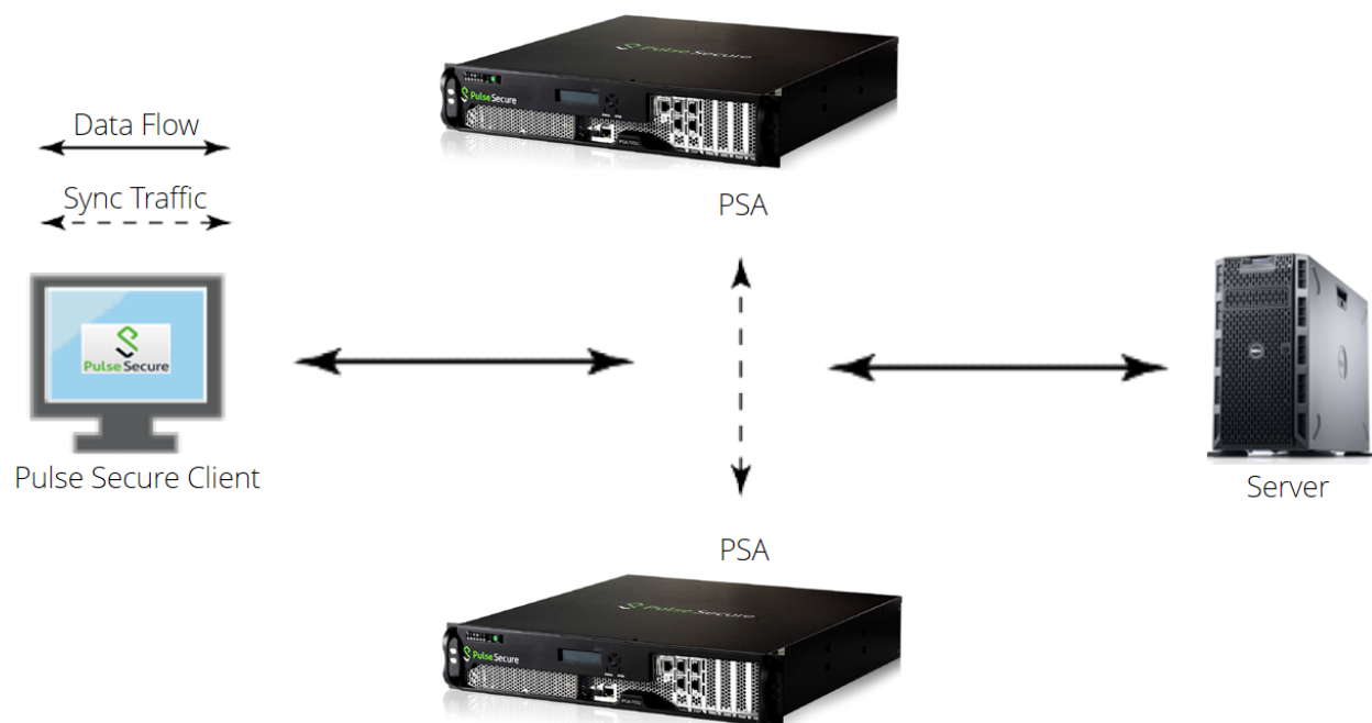
Figure 277: Clustering
