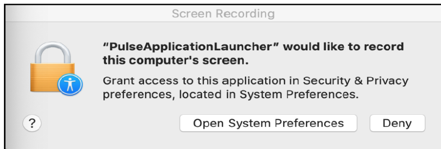
Figure 144 Screen Recording
