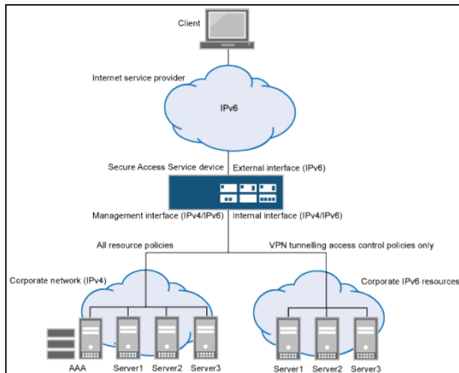
Figure 180 Dual Stack Endpoint Access Over ISP IPv6 Network
