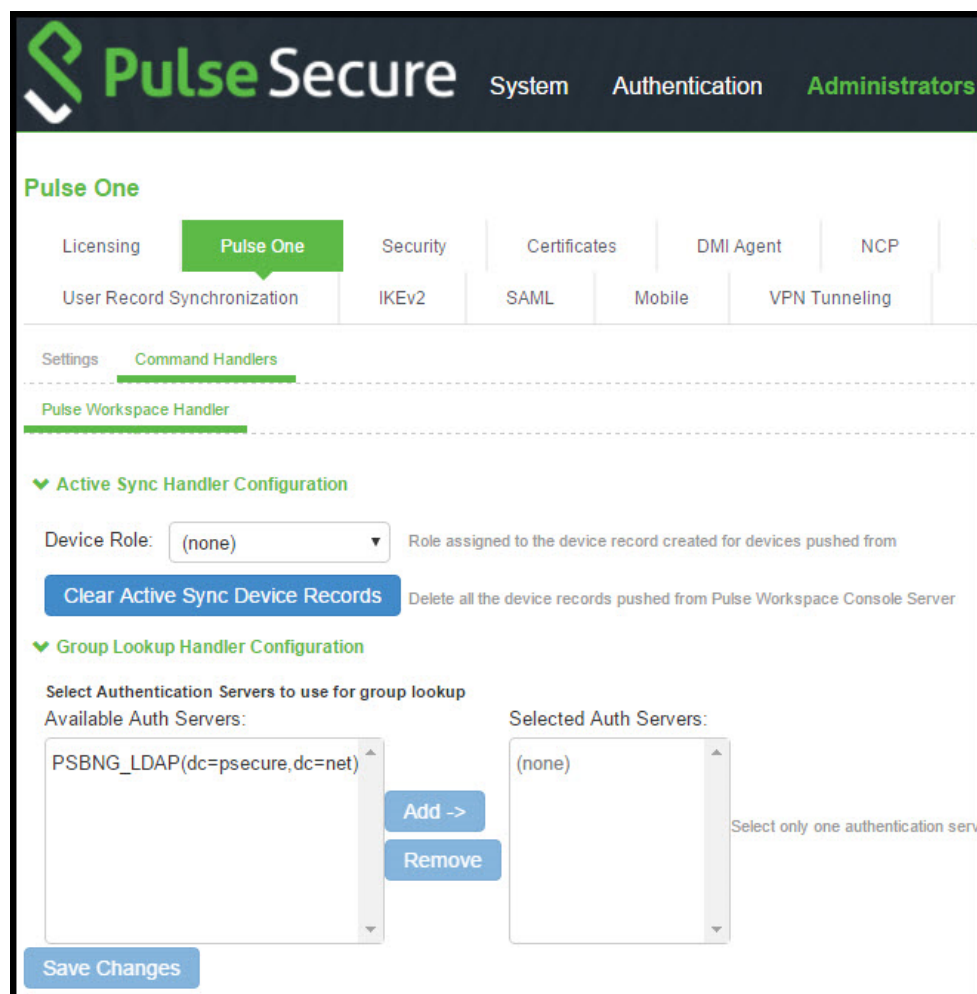
Figure 353 Pulse Workspace Handlers
