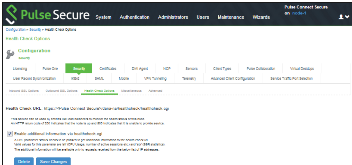
Figure 192 Health Check Security Options Configuration Page
