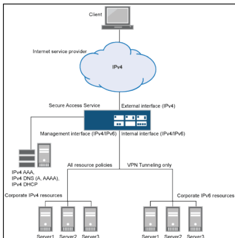
Figure 179 Dual Stack Endpoint Access Over ISP IPv4 Network
