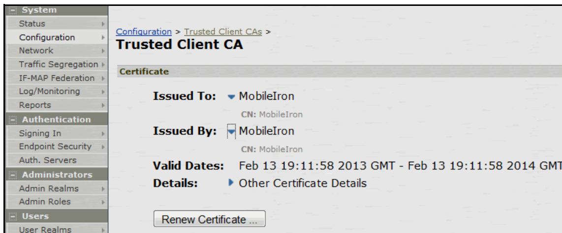
Figure 76 Trusted Client CA Configuration for MobileIron
