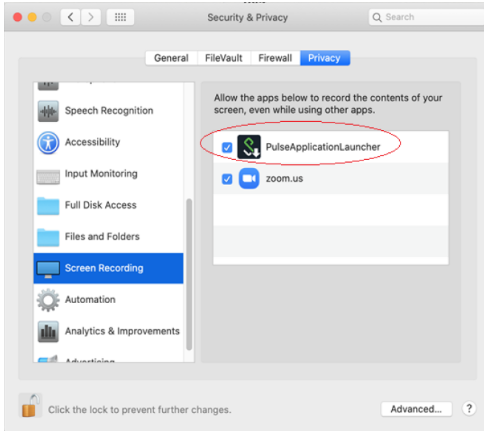
Figure 146 Screen Recording
