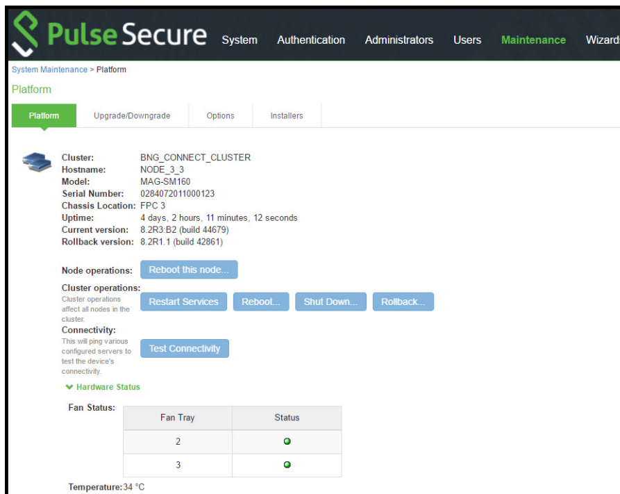
Figure 247 System Maintenance Platform Page
