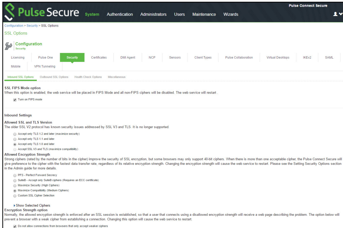
Figure 355 Enabling FIPS Level 1 Support
