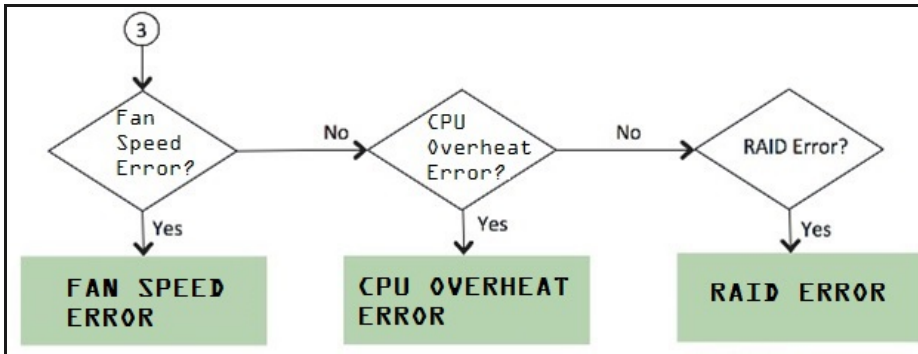
Figure 261 Error Conditions
