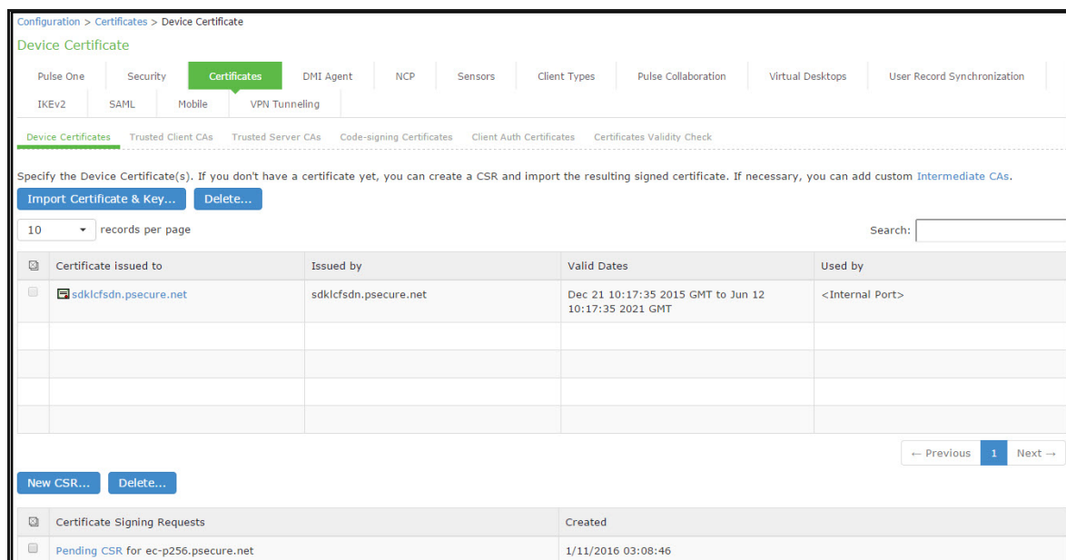
Figure 214 Pending CSR
