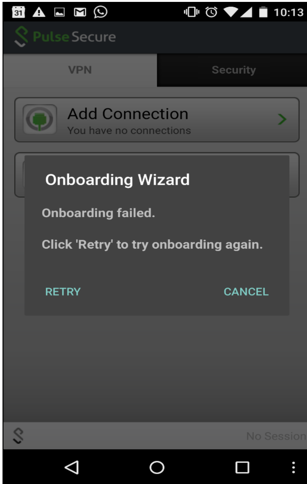
Figure 162 Error Page
