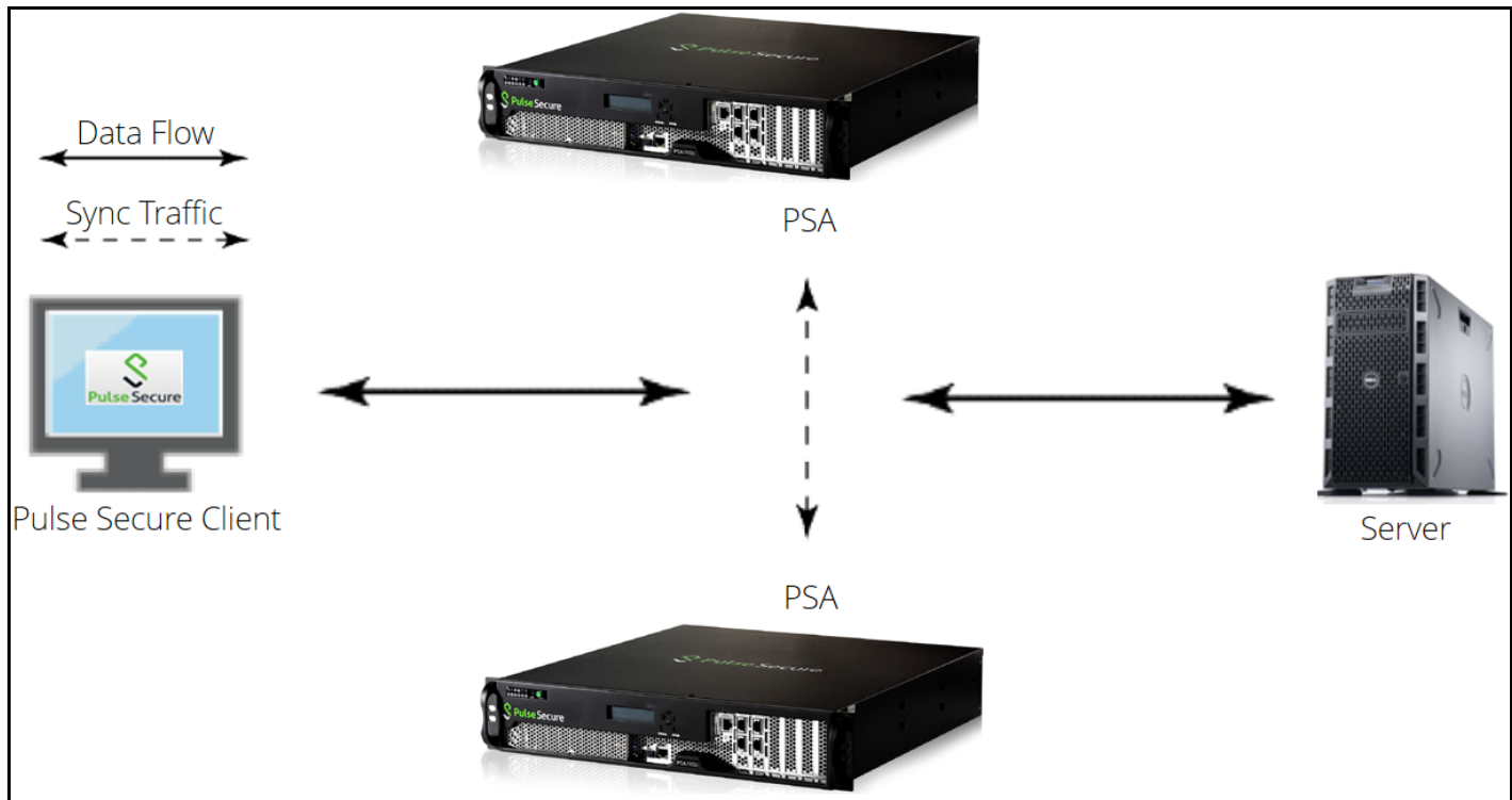
Figure 284 Clustering
