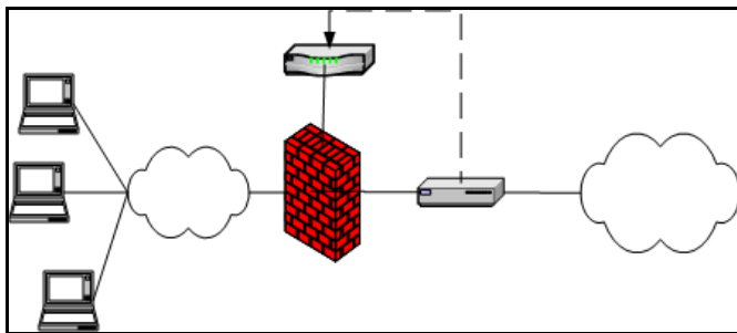
Figure 321 Pulse Connect Secure and IDP Topology Scenario 1
