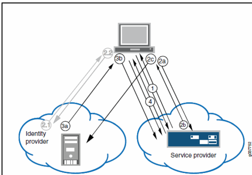
Figure 26 Connect Secure as a SAML Service Provider in a Pulse-Client-Initiated Connection
