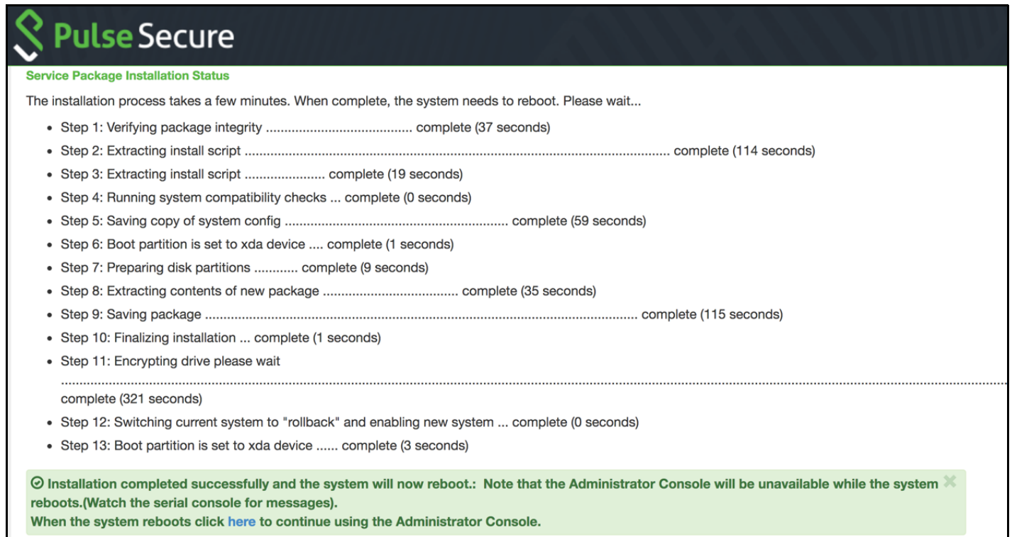
Figure 244 Software Upgrade Status Page
