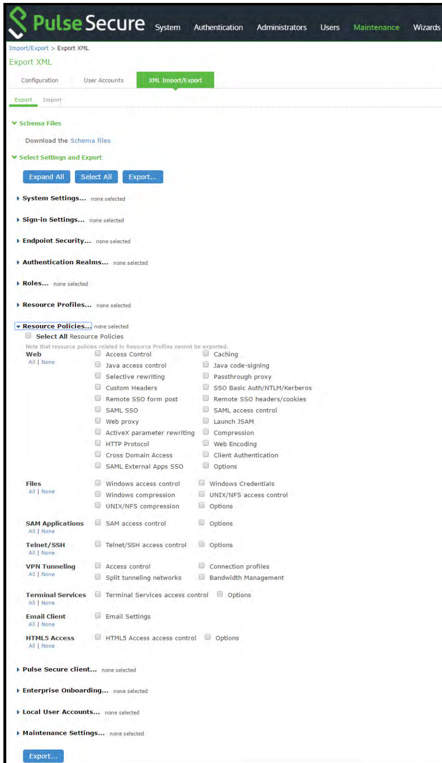
Figure 236 Export XML File Configuration Page - Pulse Connect Secure
