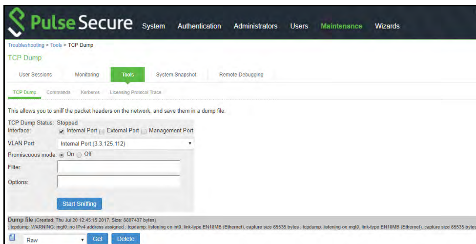
Figure 276 TCP Dump Configuration Page - Pulse Connect Secure
