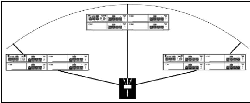
Figure 289 Active/Passive Deployment
