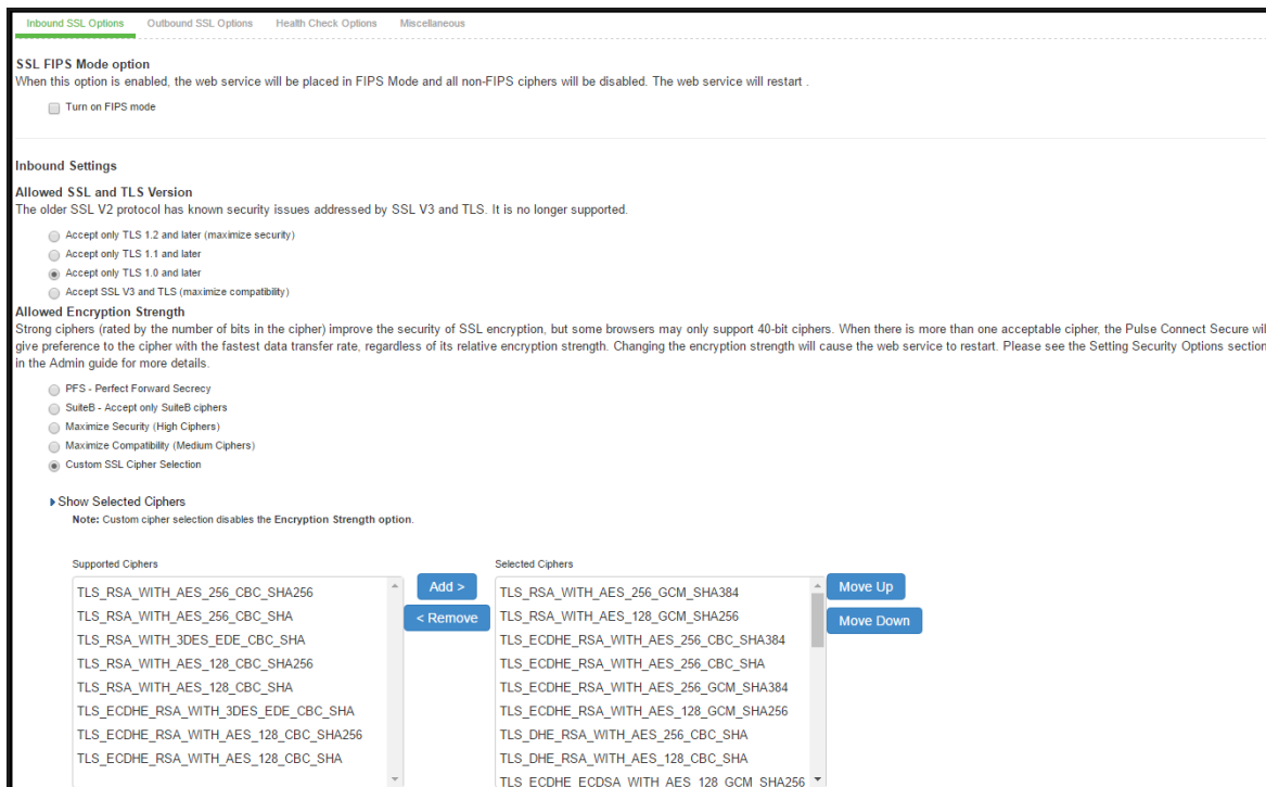
Figure 219 Supported Ciphers and Selected Ciphers Panels
