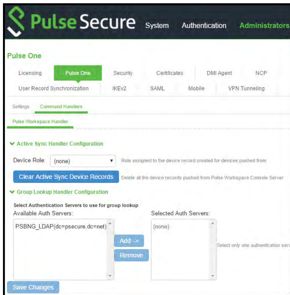
Figure 356 Pulse Workspace Handlers
