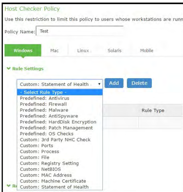
Figure 105 Rule Settings for Host Checker Policy
