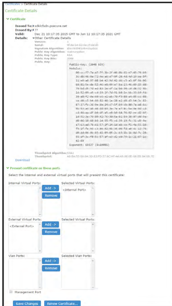
Figure 171 Pulse Connect Secure Certificate Details Page
