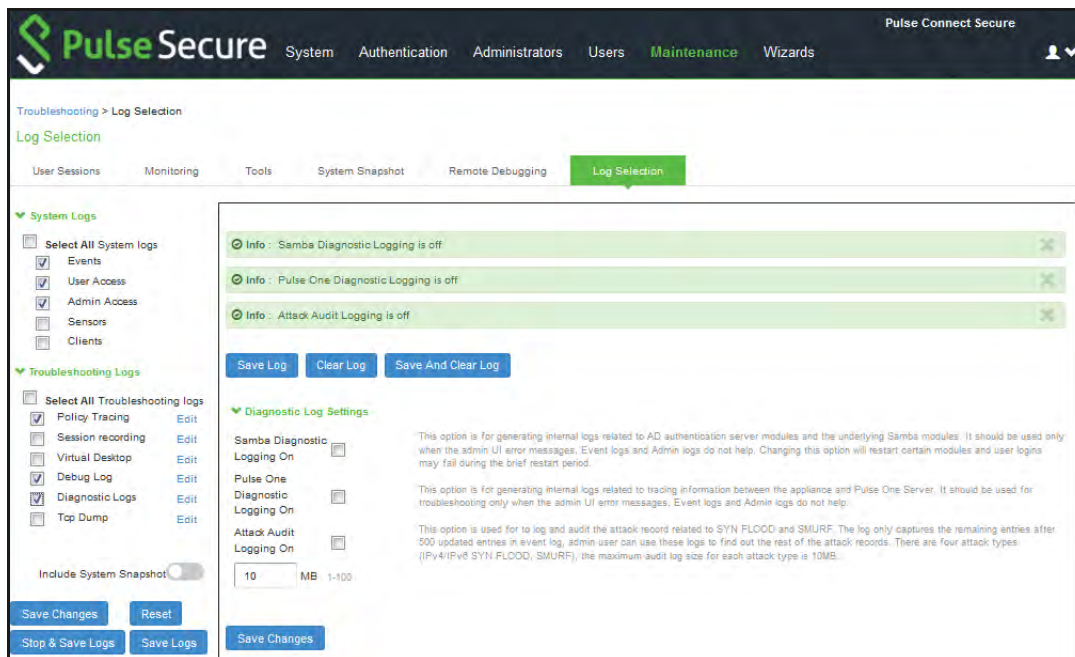
Figure 286 Log Selection Page
