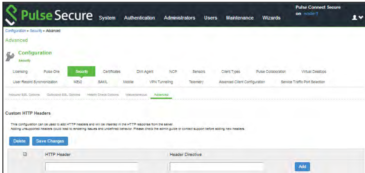
Figure 196 Custom HTTP Headers Page
