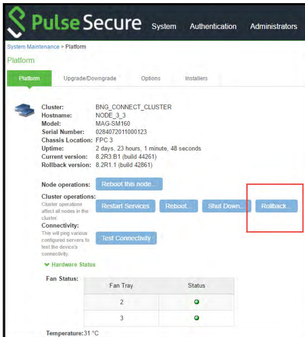
Figure 247 System Maintenance Platform Page
