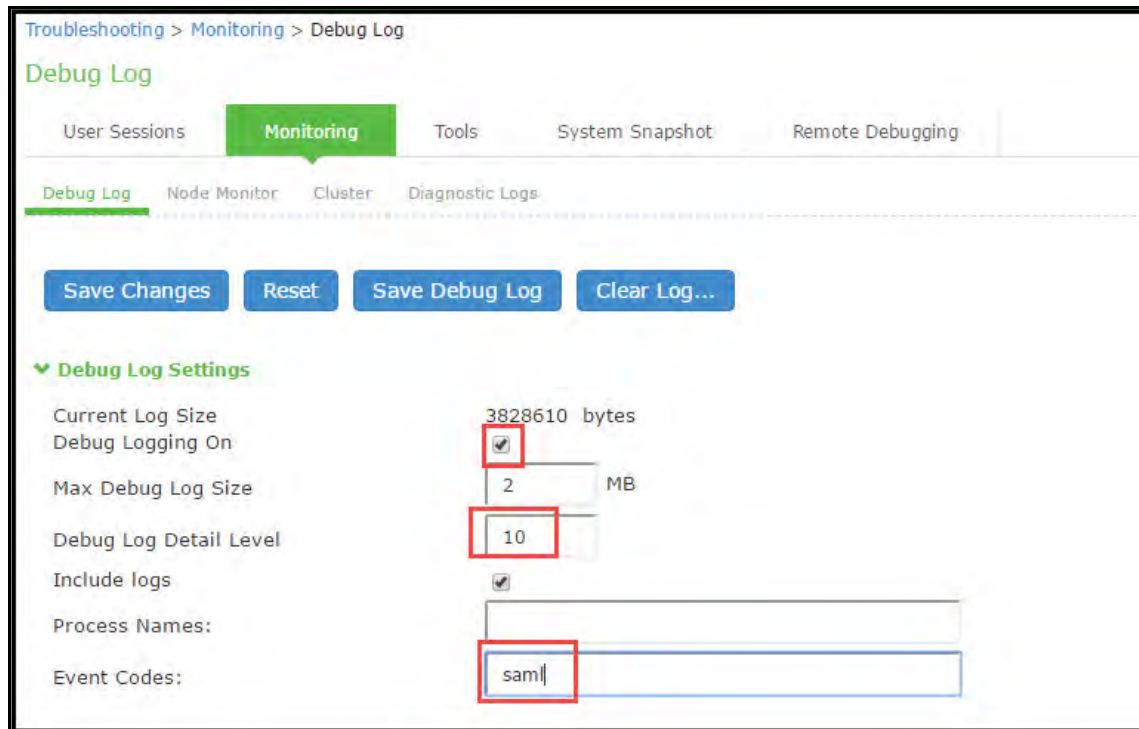
Figure 43 Debug Log Page
