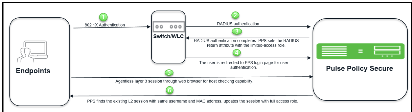
Figure 111 Agentless Host Checking with Native Supplicant
