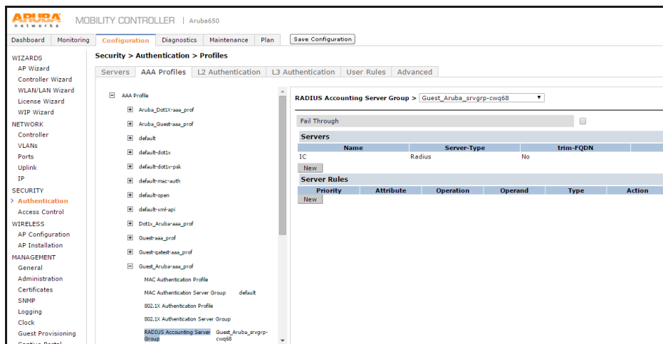
Figure 503 RADIUS Accounting Server Group
