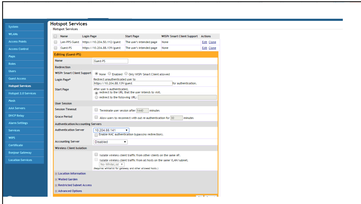
Figure 529 ZoneDirector Hotspot Services
