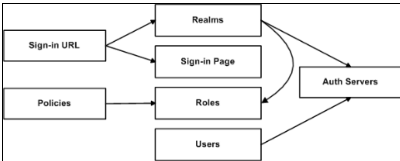
Figure 617 Object Referential Integrity Constraints
