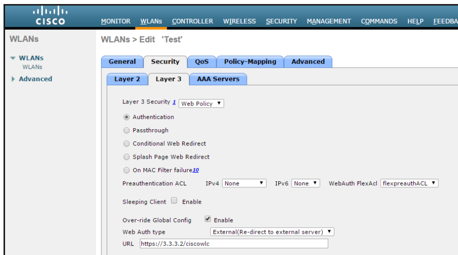
Figure 456 WLAN – Layer 3 settings
