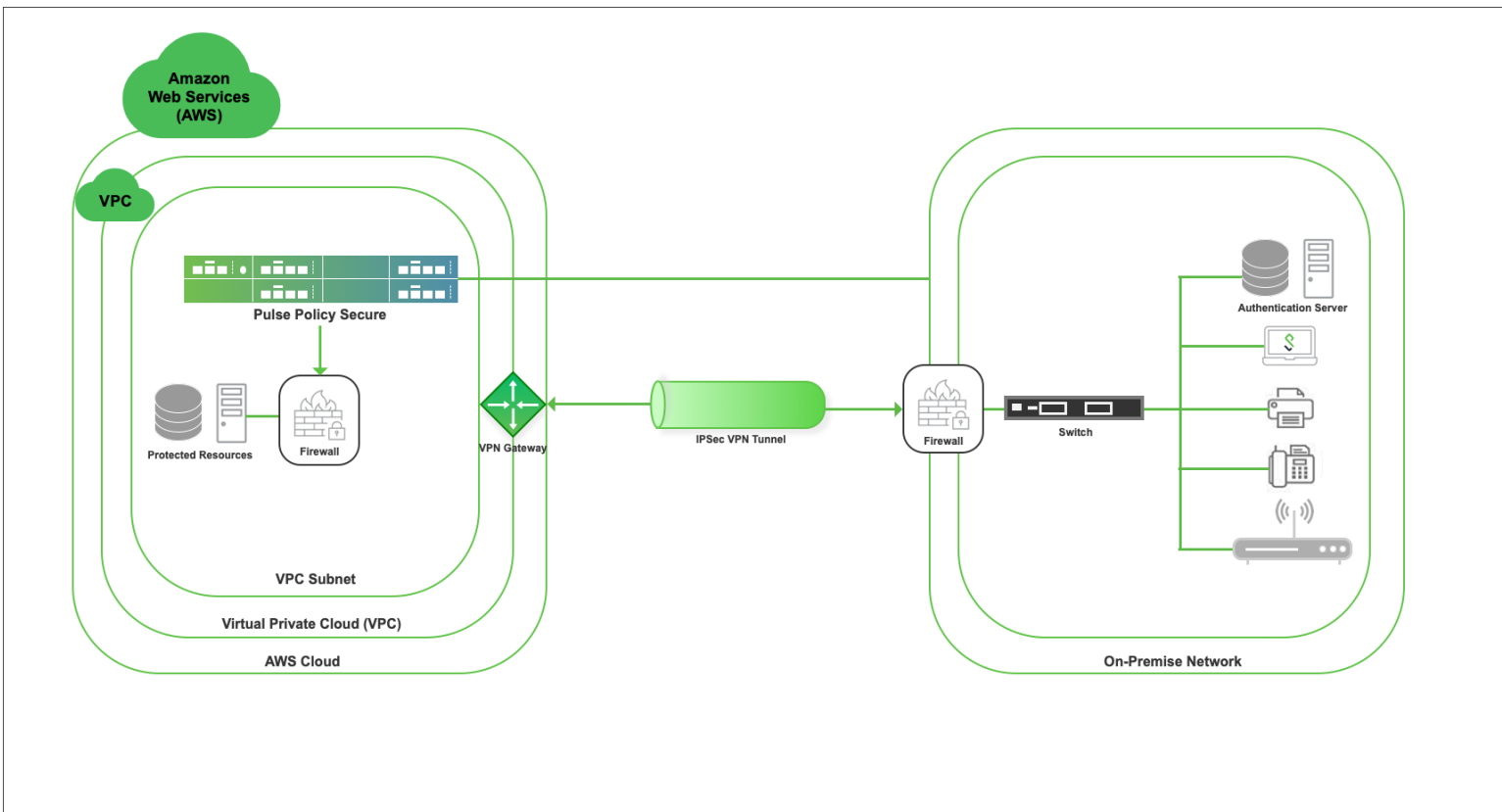
Figure 1: Pulse Policy Secure on AWS
