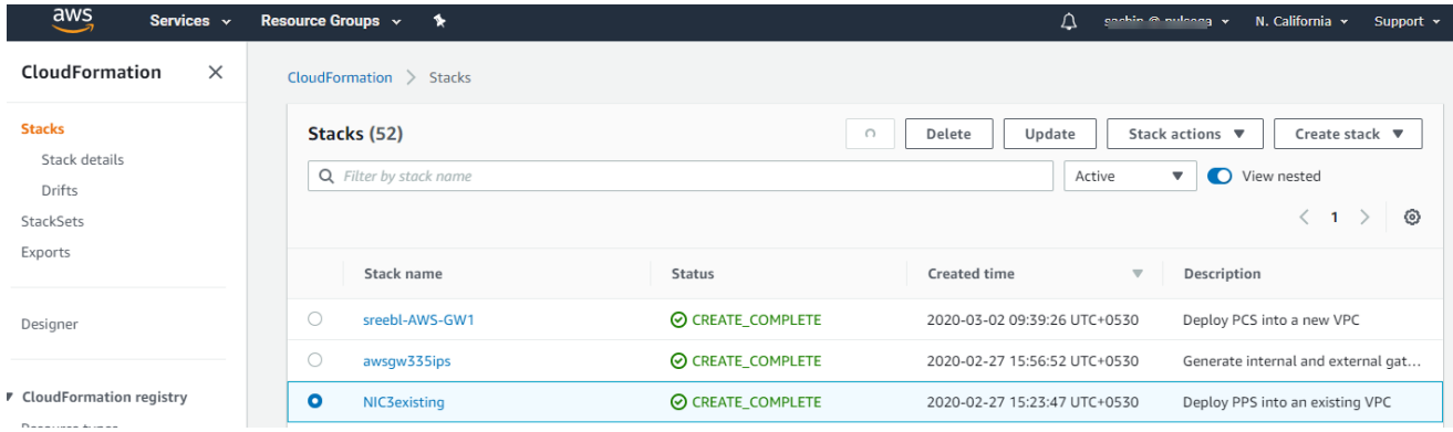
Figure 23: Delete Stack
