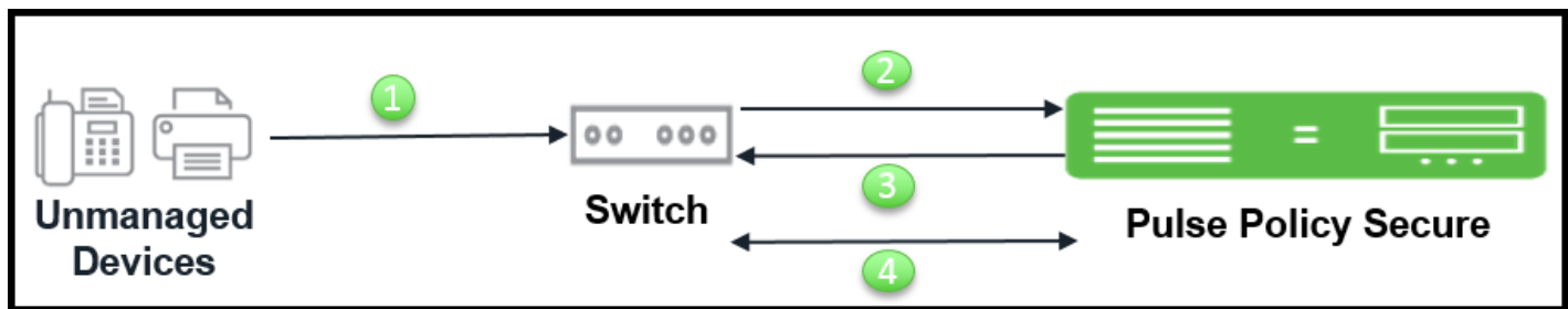
Figure 83 Policy Enforcement using SNMP for unmanaged devices
