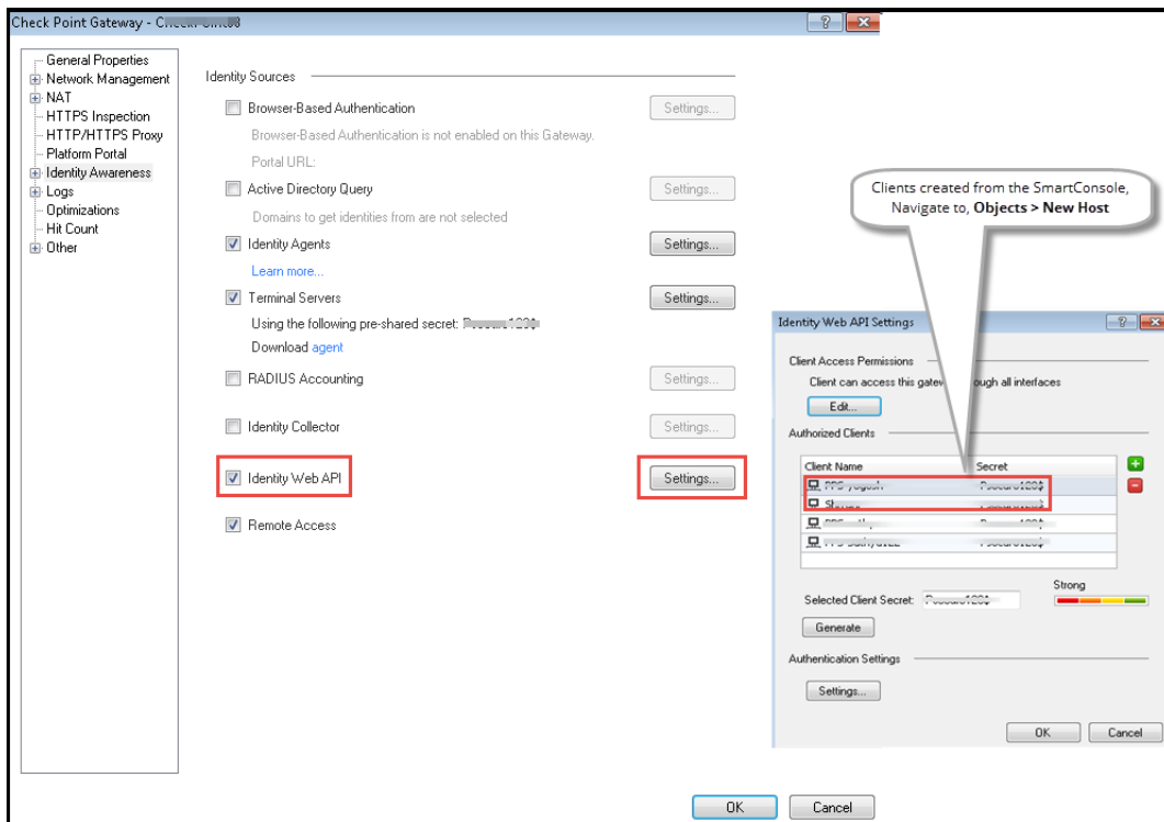
Figure 139 Identity Awareness
