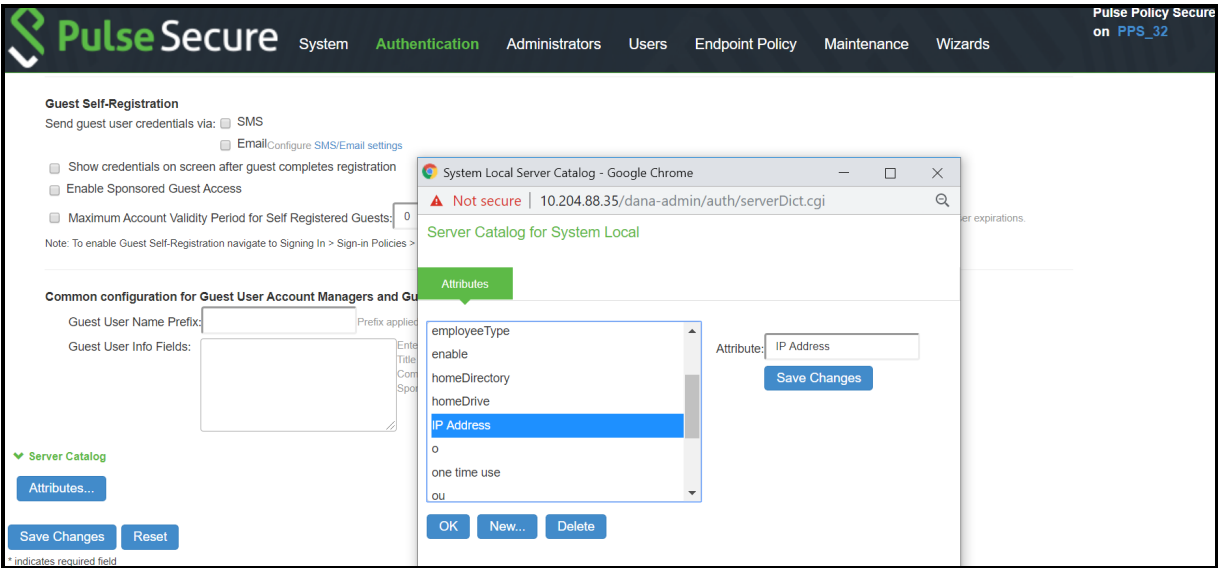
Figure 364 Return Attributes
