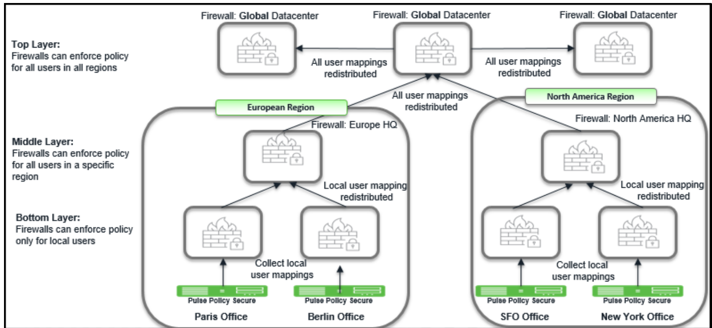
Figure 130 Check Point with PPS
