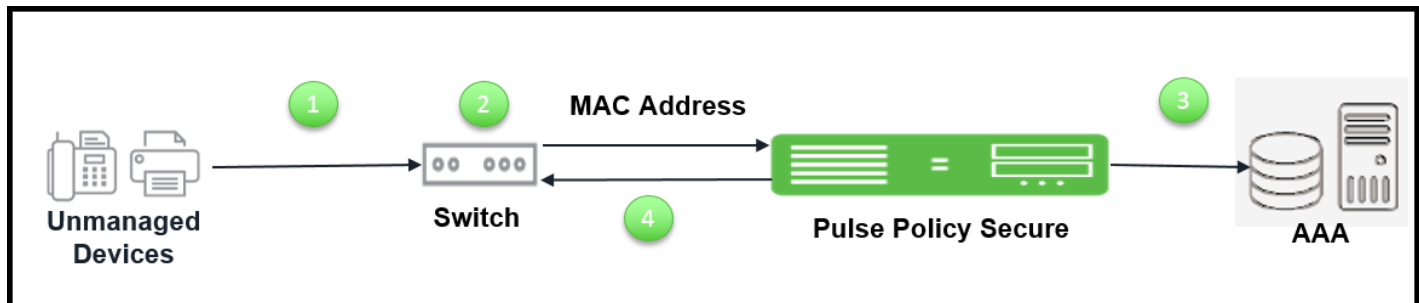
Figure 101 PPS Deployment using Local MAC Authentication Server
