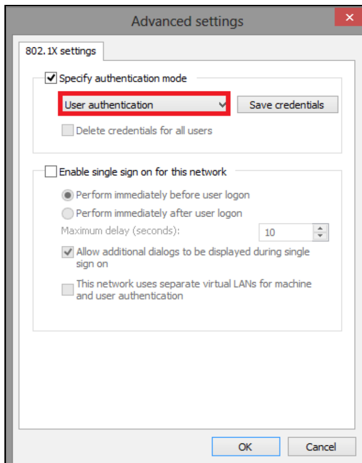
Figure 122 Advanced Settings
