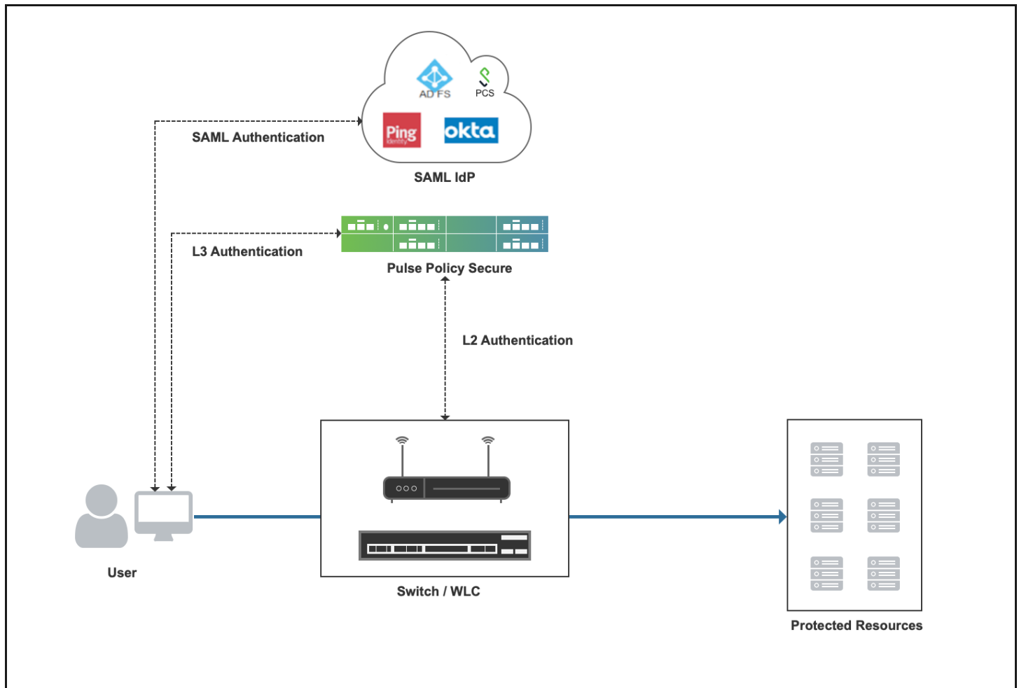
Figure 376 Authentication Deployment Diagram
