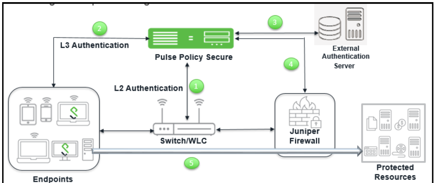
Figure 178 Deployment using SRX Firewall
