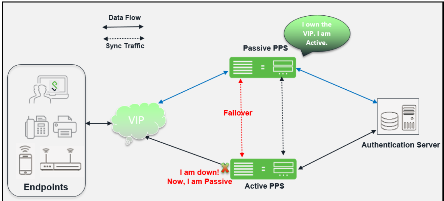
Figure 612 Active/Passive Cluster
