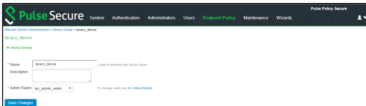
Figure 338 TACACS+ Device Group
