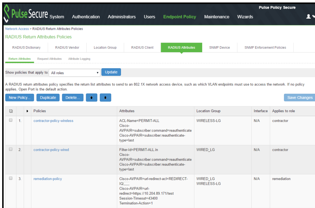
Figure 113 RADIUS Return Attributes for CoA
