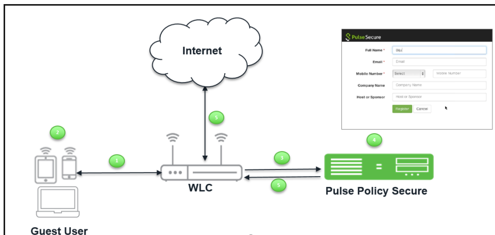
Figure 351 Guest Access using WLC
