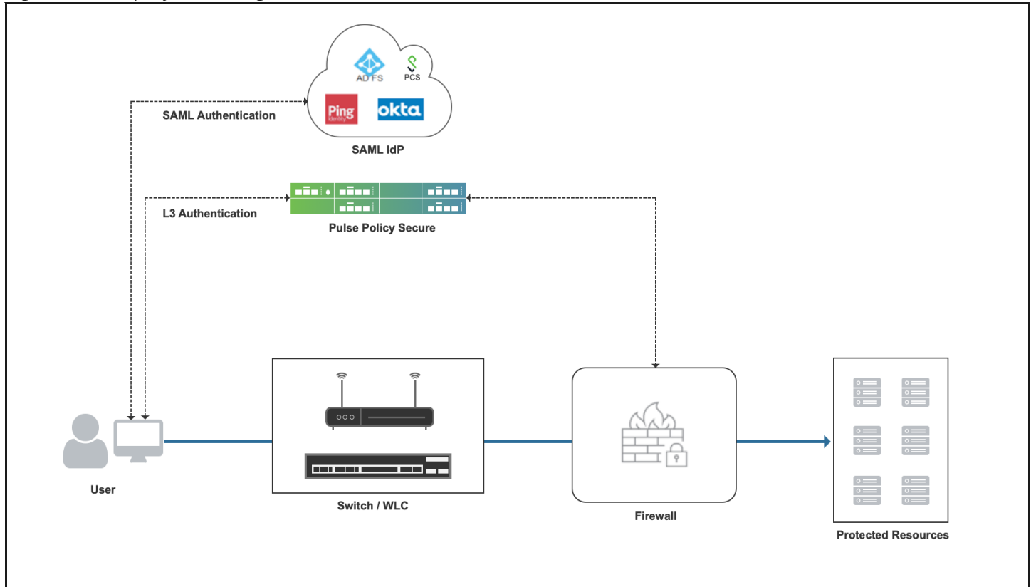
Figure 318 Deployment diagram
