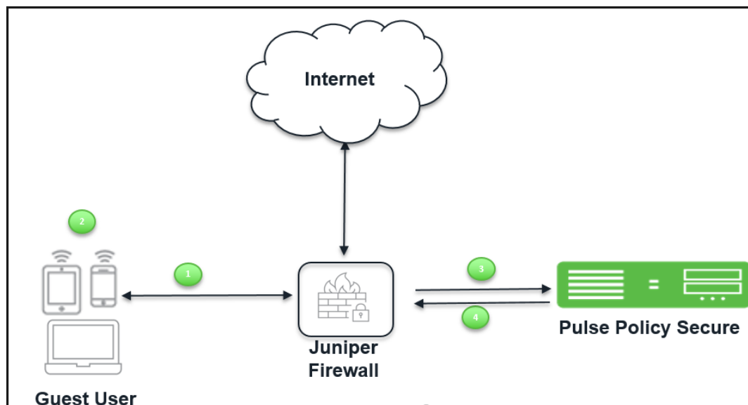
Figure 352 Guest Access using SRX/EX
