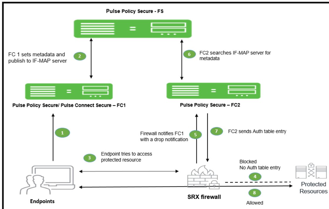
Figure 189 Access Control in the federated enterprise using IF-MAP
