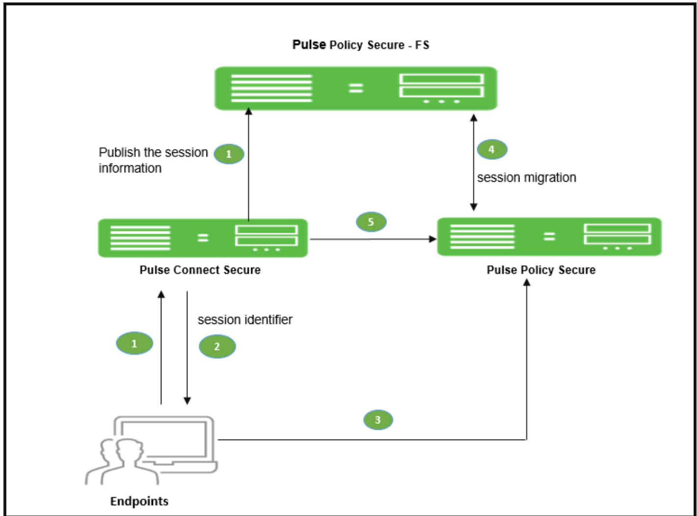
Figure 190 Session Migration across PCS and PPS
