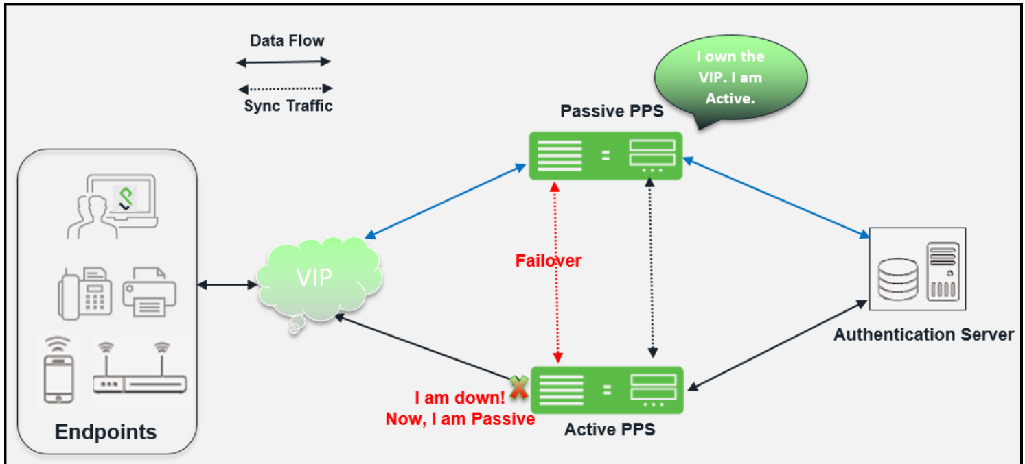
Figure 549 Active/Passive Cluster
