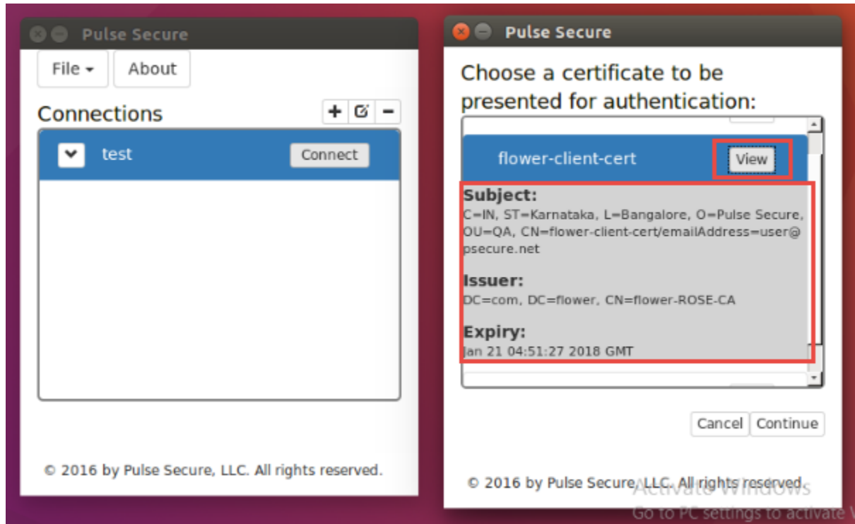
Figure 23 Certs_details_onclicking view
