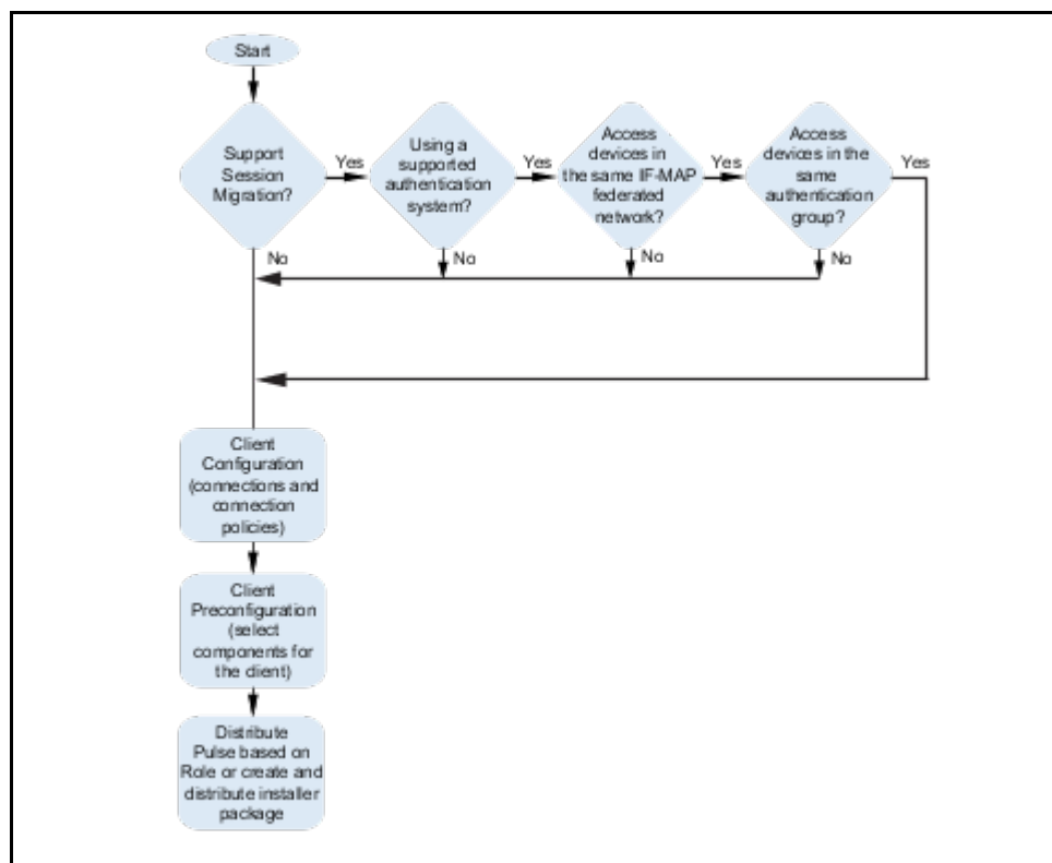
Figure 108 Requirements for Pulse Client Session Migration
