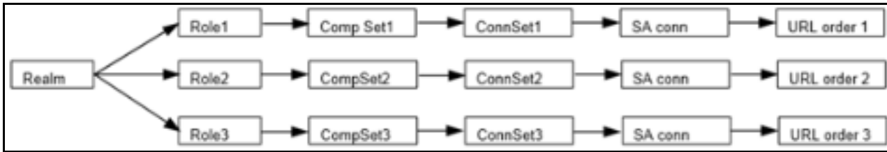
Figure 25 Mapping URL Lists to Users
