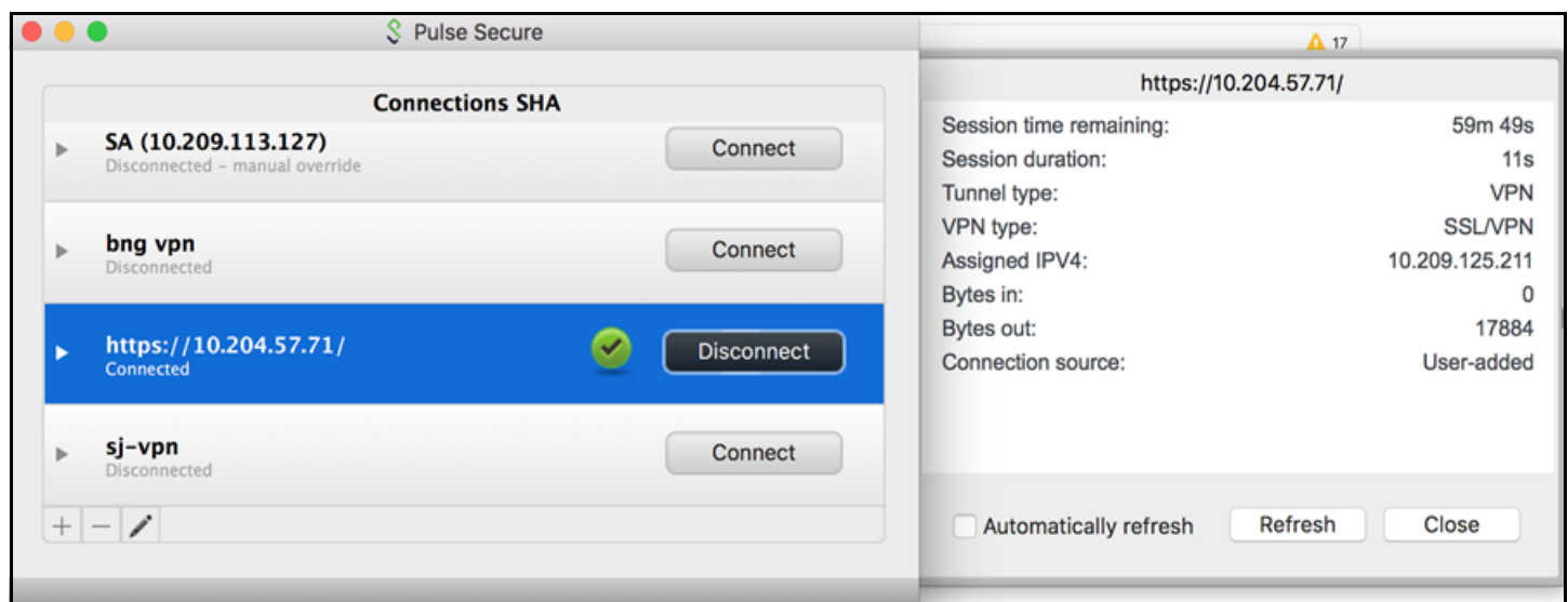
Figure 7 Pulse Client for Mac client Interface
