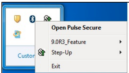
Figure 70 Step-Up connection – Pulse Client Tray icon
