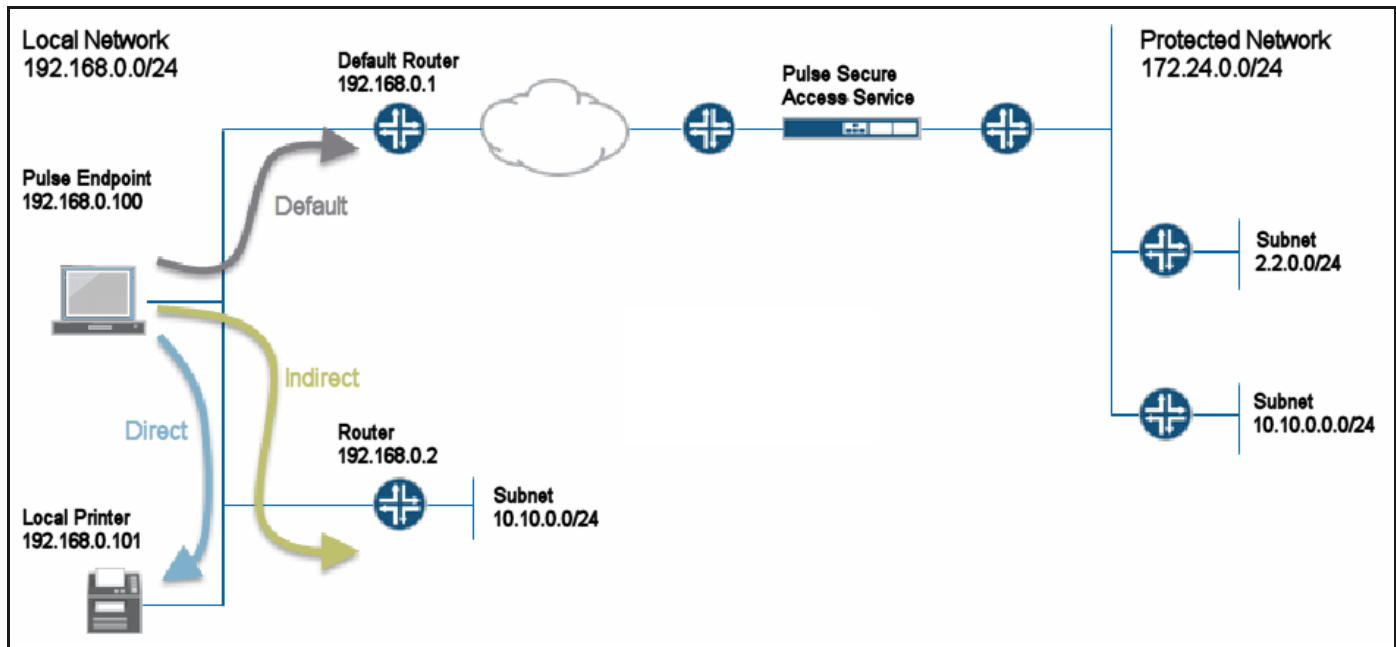
Figure 54 Pulse Client Split Tunneling
