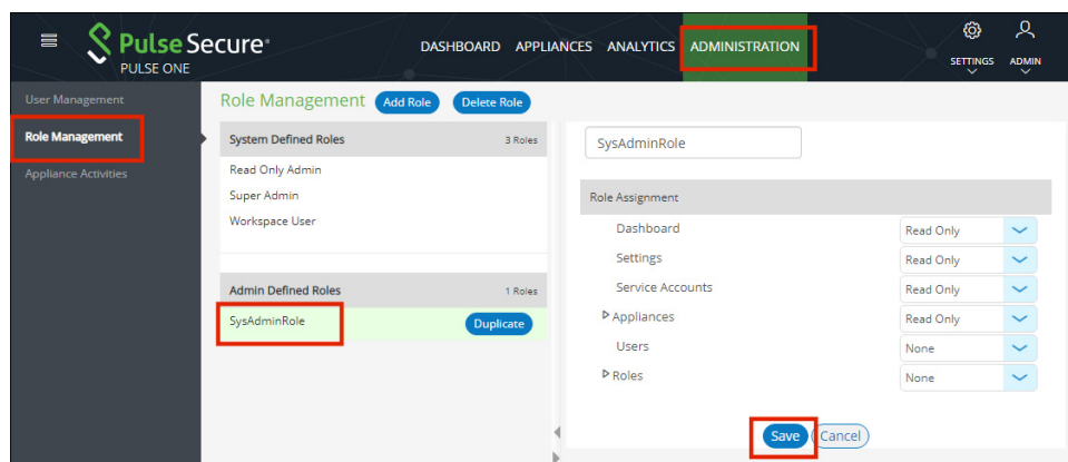
FIGURE 152 Modify Role
