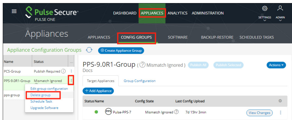
FIGURE 138 Delete Group
