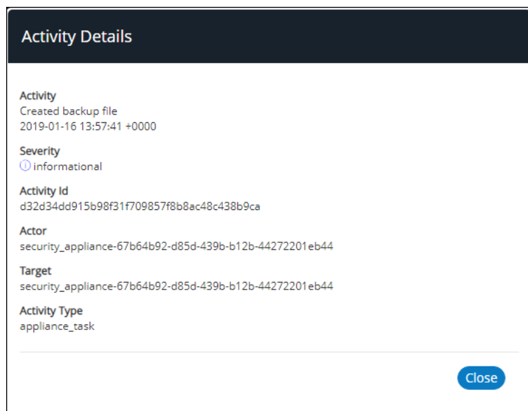
FIGURE 146 Activity Details
