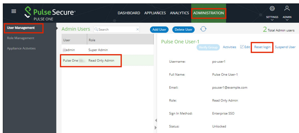
FIGURE 149 Reset Login
