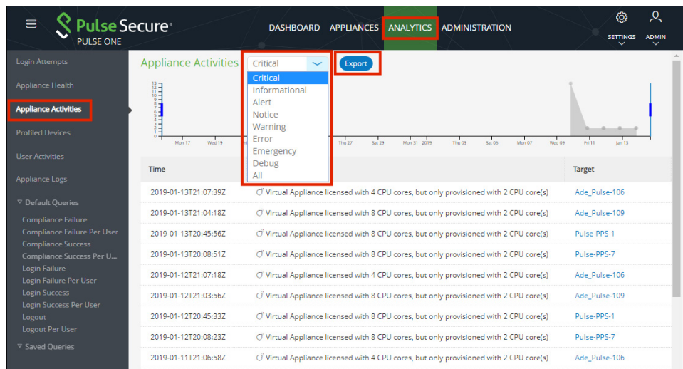
FIGURE 142 Appliance Activities
