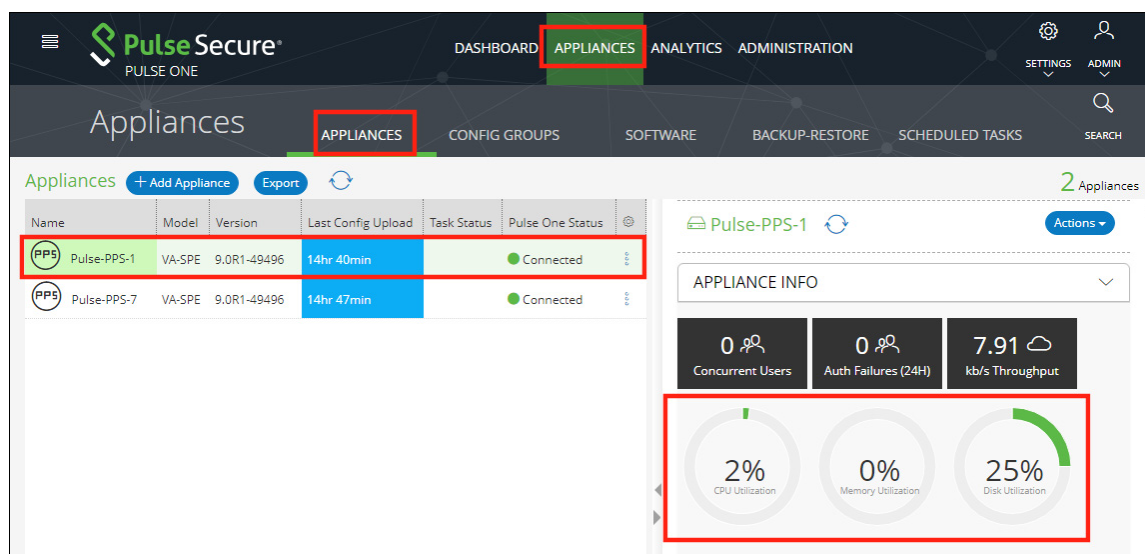
FIGURE 85 Appliance Health
