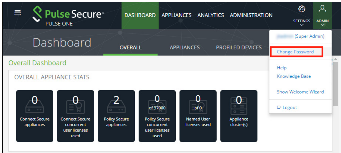
FIGURE 14 Change Password
