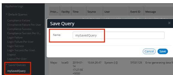
FIGURE 144 Save Query
