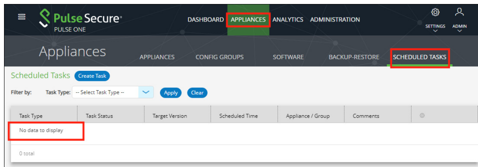
FIGURE 122 Scheduled Tasks
