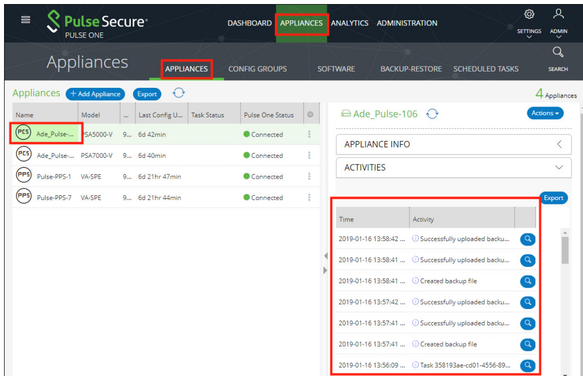
FIGURE 129 Activities Details
