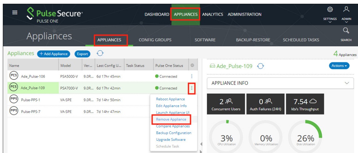
FIGURE 134 Remove Appliance
