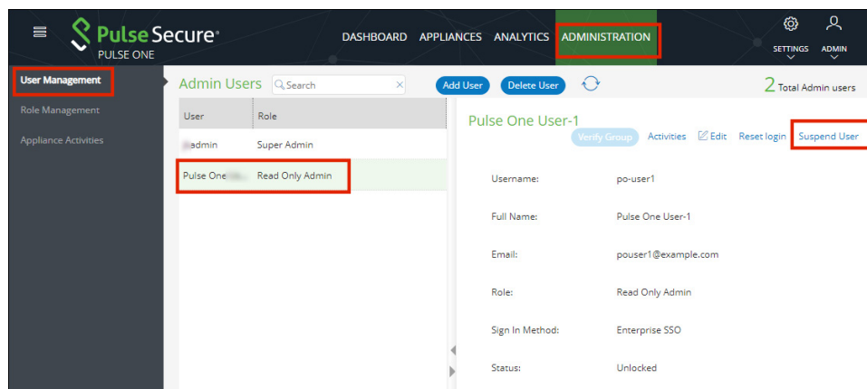
FIGURE 150 Suspend User
