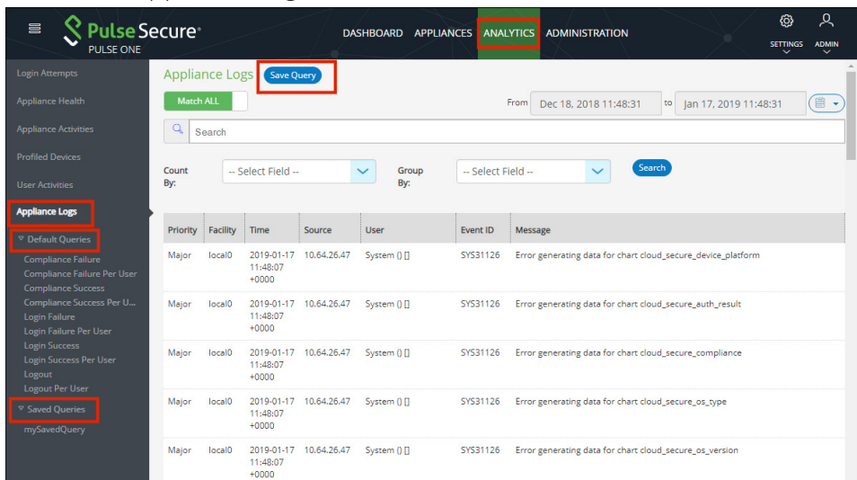
FIGURE 143 Appliance Logs
