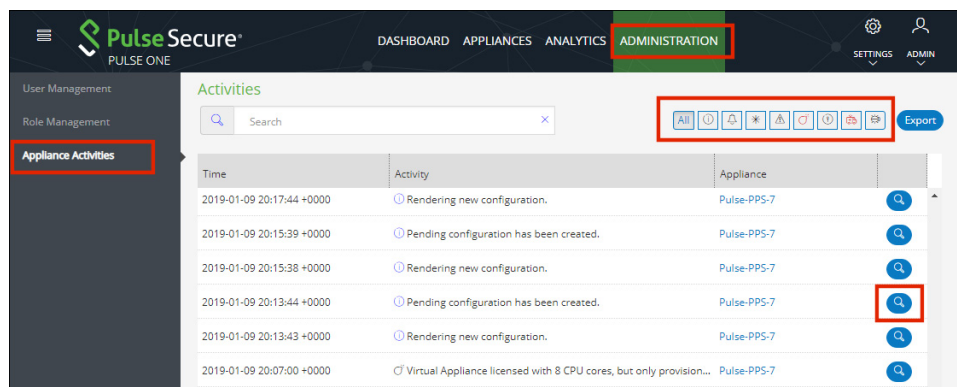
FIGURE 145 Filter Activities
