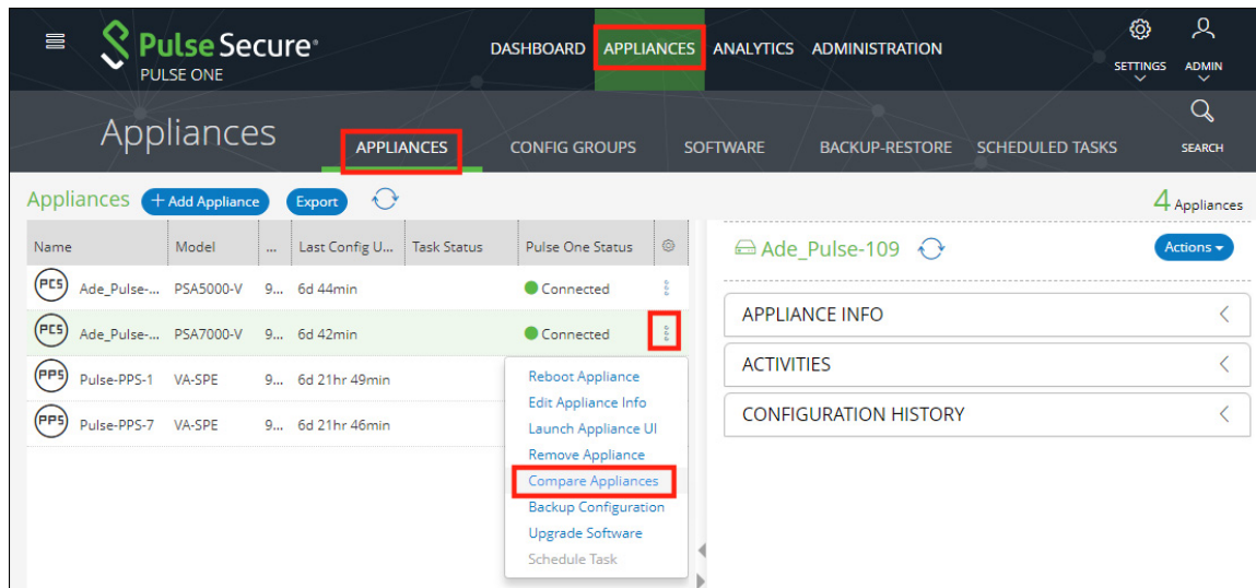
FIGURE 131 Compare Appliances
