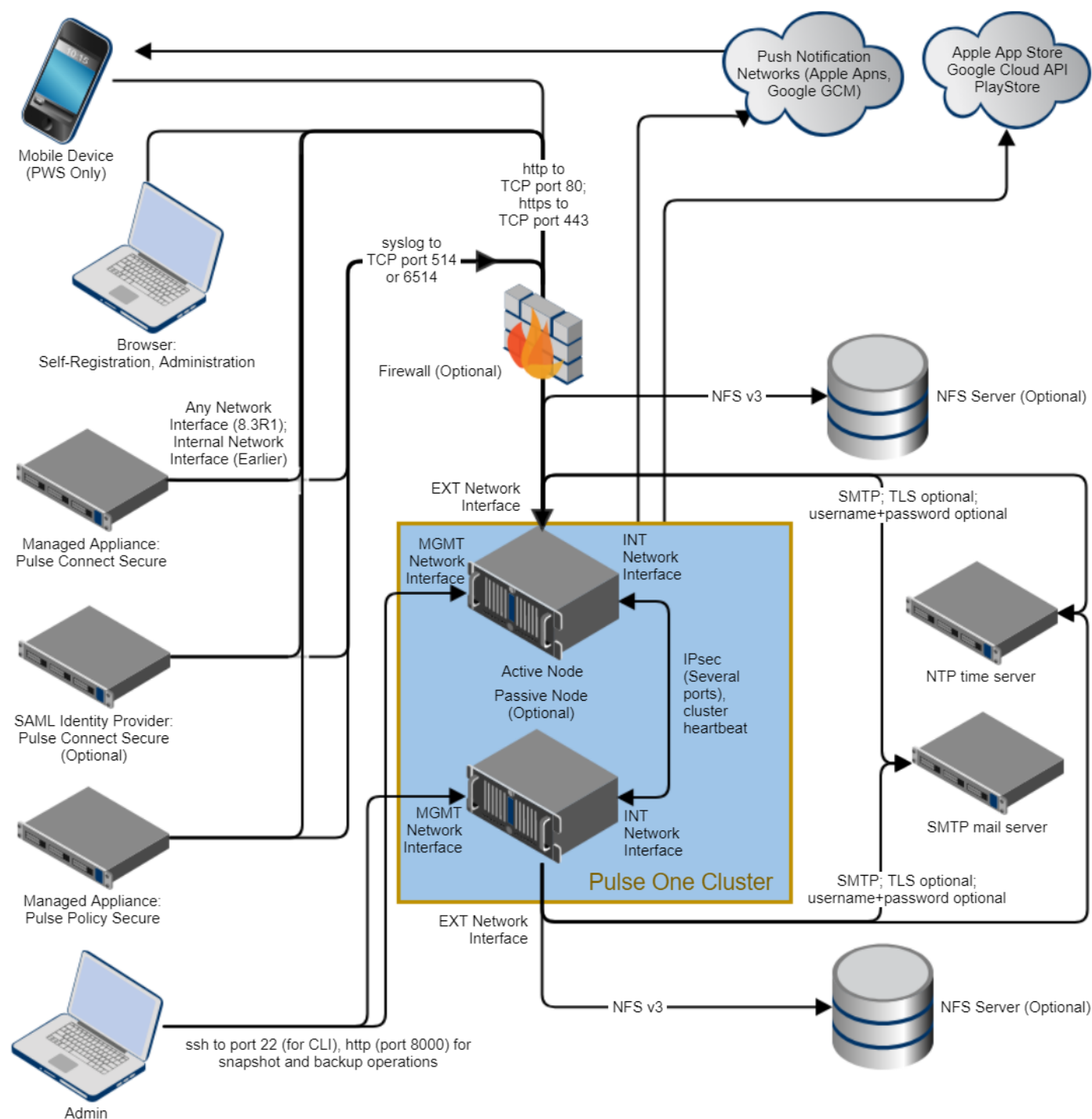
FIGURE 2 Pulse One Appliance Architecture
