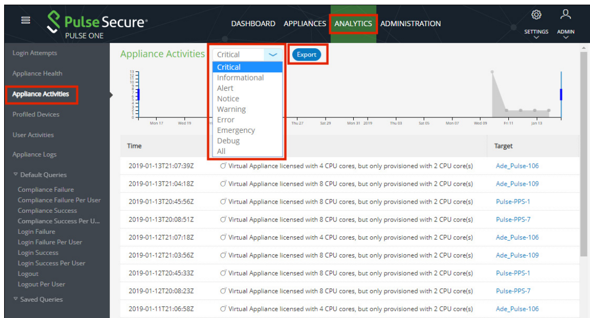
FIGURE 152 Appliance Activities
