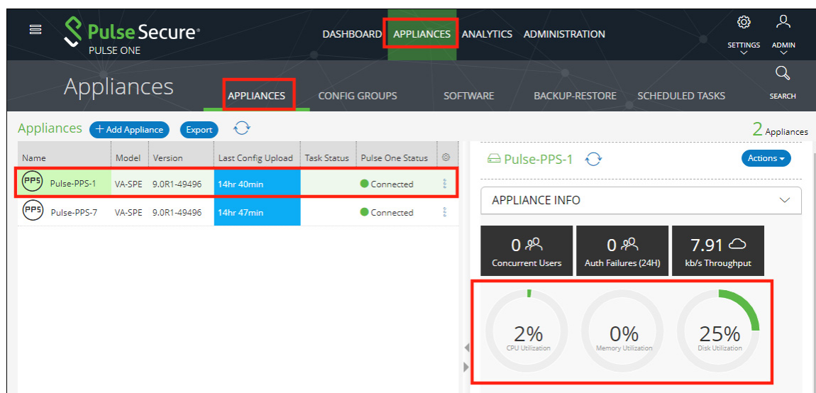
FIGURE 92 Appliance Health
