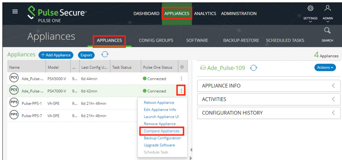
FIGURE 142 Compare Appliances
