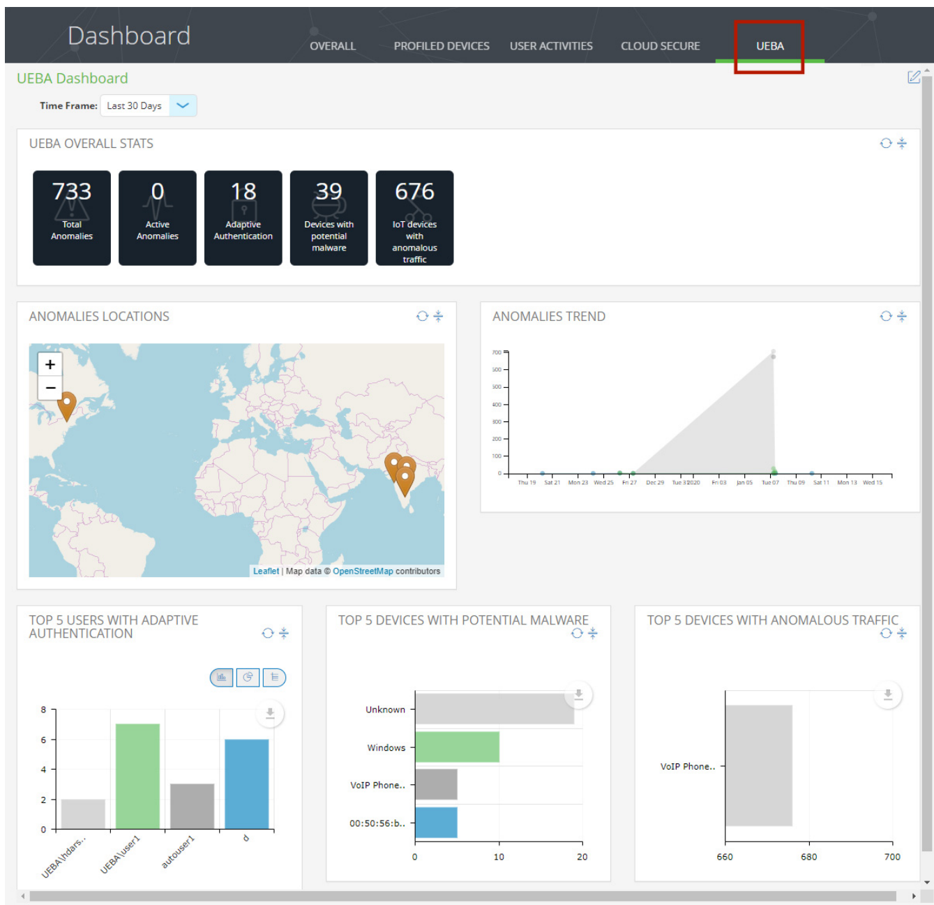
FIGURE 27 UEBA Dashboard
