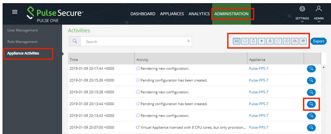
FIGURE 159 Filter Activities
