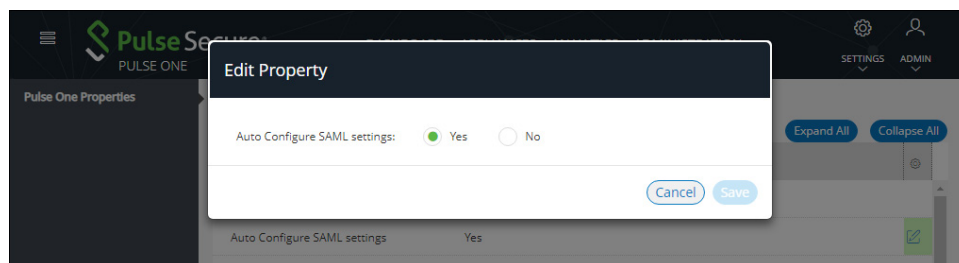
FIGURE 168 Edit Properties
