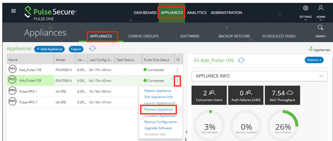
FIGURE 145 Remove Appliance
