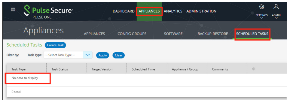
FIGURE 129 Scheduled Tasks
