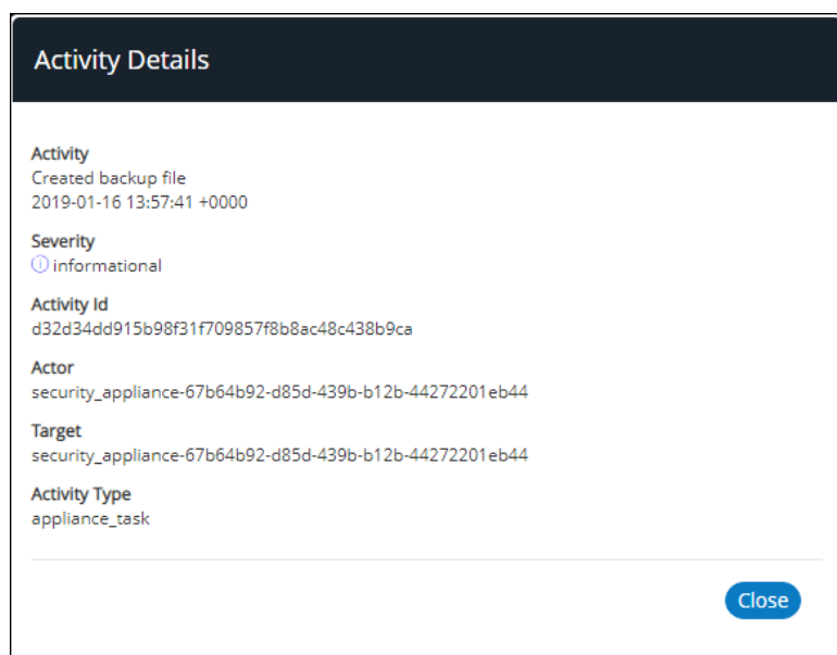
FIGURE 160 Activity Details
