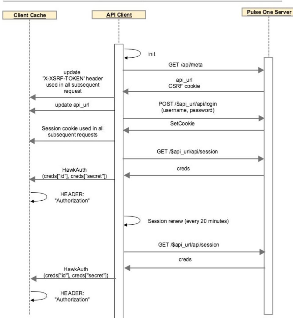
APIClientauthenticationsequence
