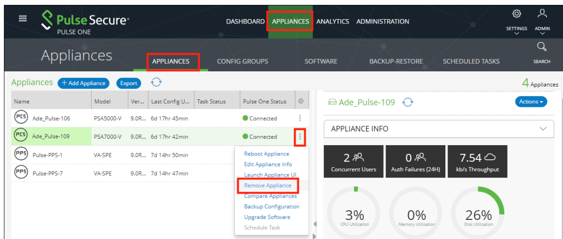
FIGURE 148 Remove Appliance
