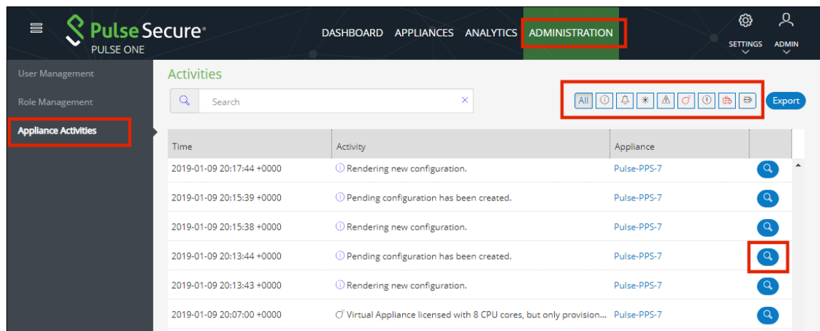
FIGURE 162 Filter Activities
