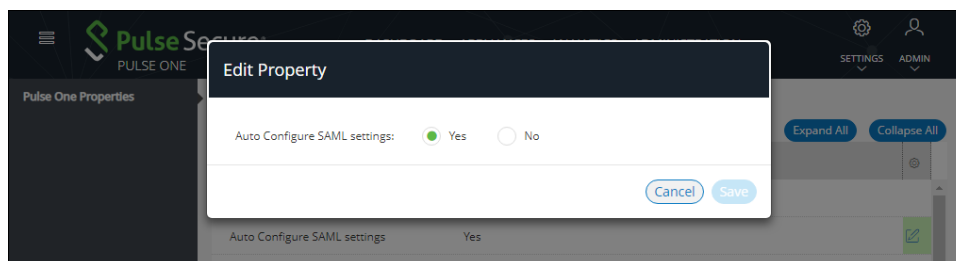
FIGURE 171 Edit Properties
