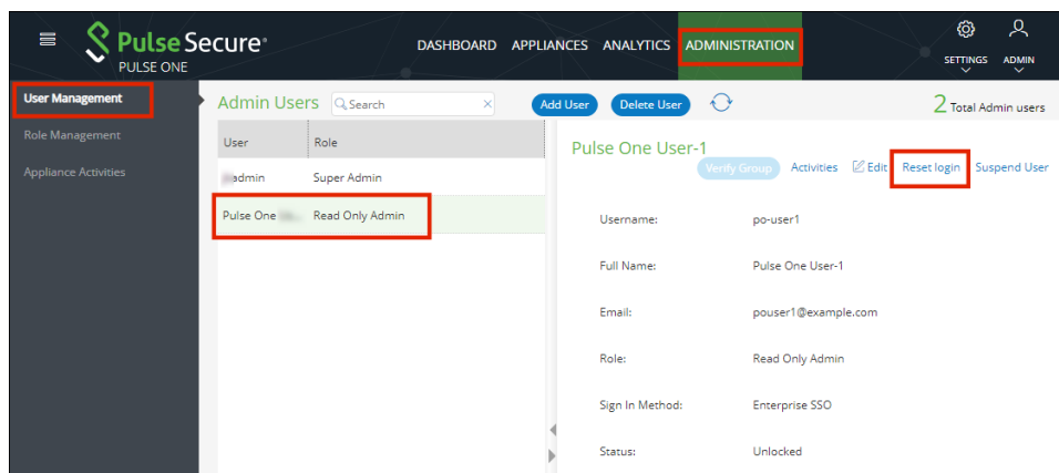
FIGURE 166 Reset Login
