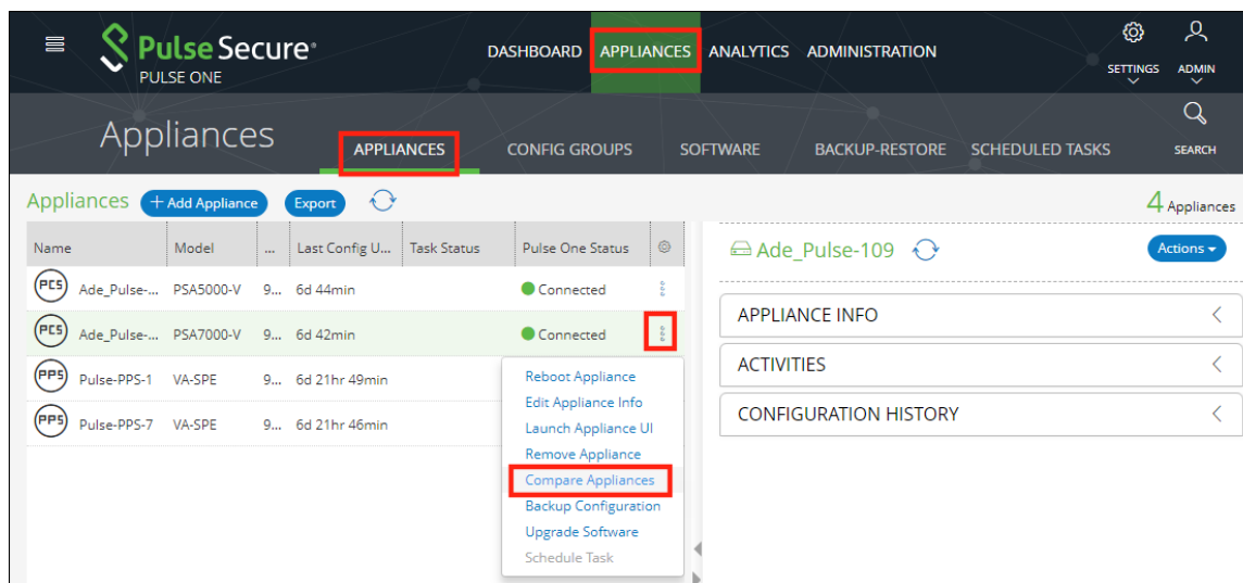
FIGURE 145 Compare Appliances
