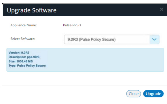
FIGURE 127 Upgrade Software
