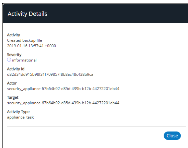
FIGURE 163 Activity Details
