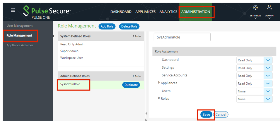
FIGURE 169 Modify Role
