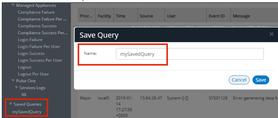
FIGURE 160 Save Query
