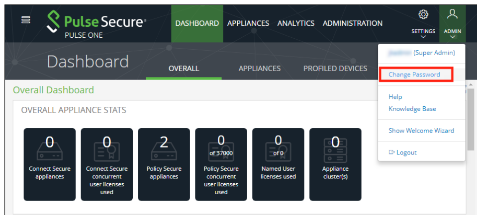
FIGURE 14 Change Password
