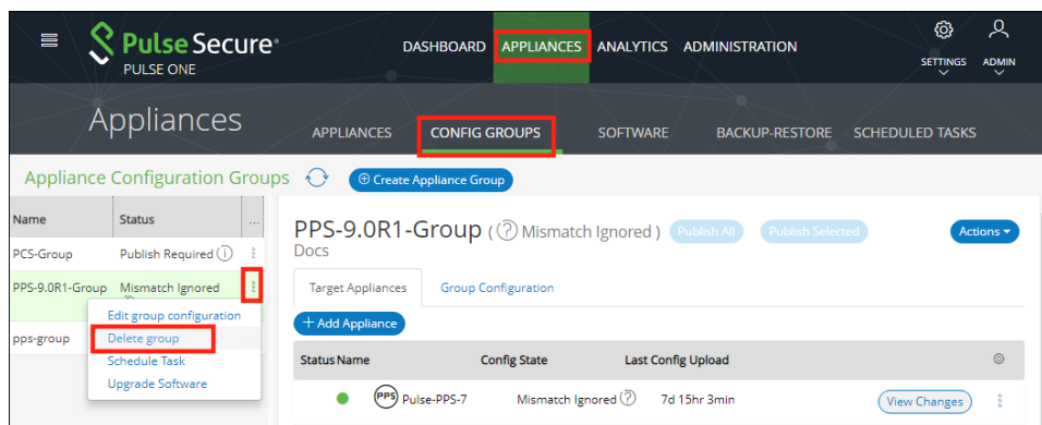
FIGURE 152 Delete Group
