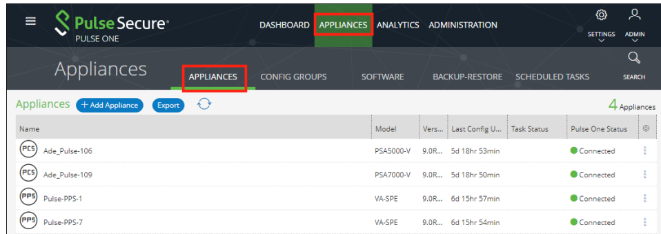
FIGURE 126 Available Appliances
