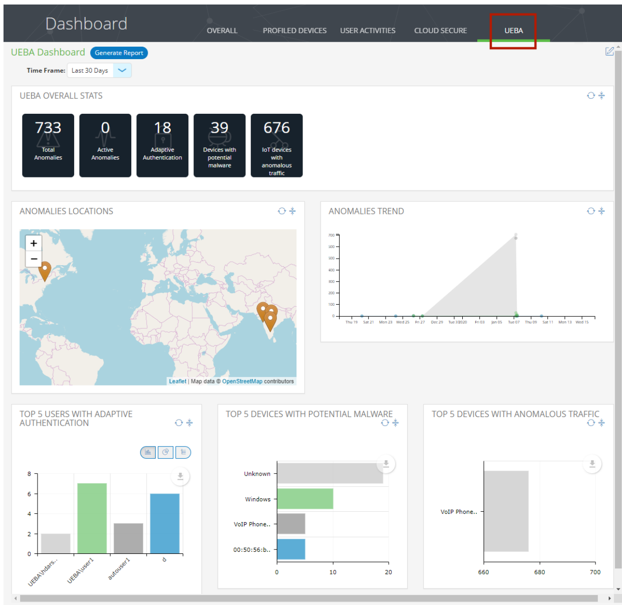
FIGURE 27 UEBA Dashboard
