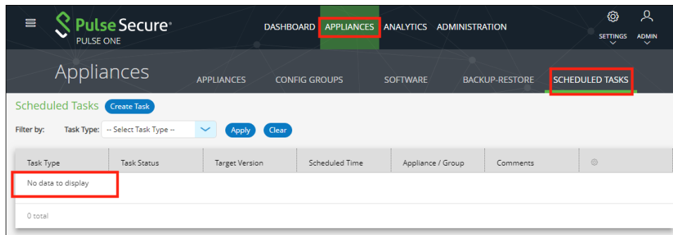
FIGURE 132 Scheduled Tasks
