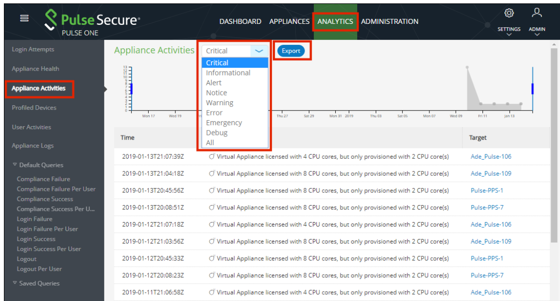
FIGURE 155 Appliance Activities
