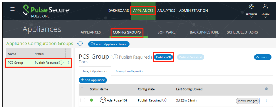
FIGURE 115 Publish All
