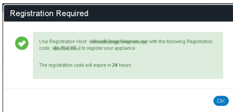
FIGURE 41 Registration Required
