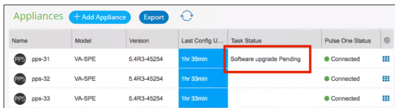
FIGURE 128 Upgrade Pending
