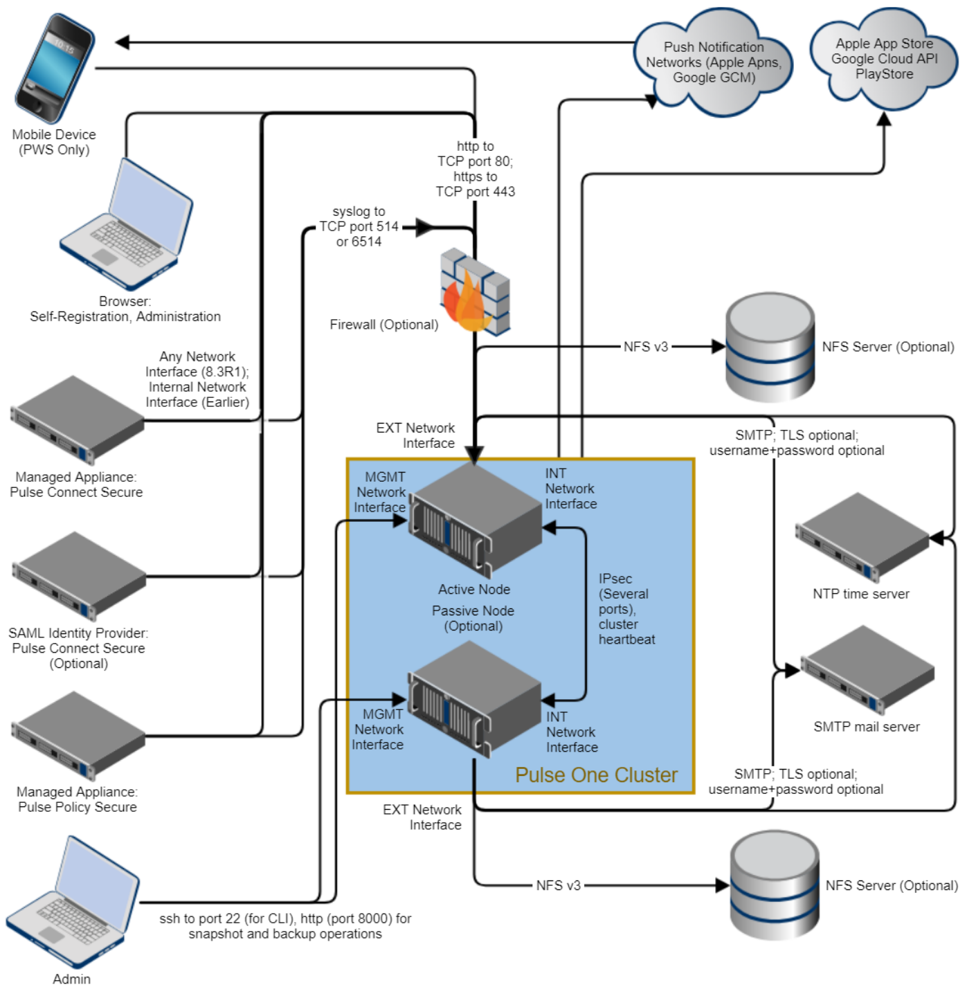
FIGURE 1 Pulse One Appliance Architecture
