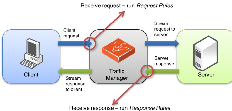
Figure 2-3. Processing rules in TrafficScript
