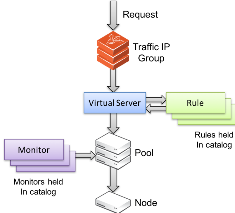
Figure 1-1. Analyzing and managing traffic using TrafficScript rules
