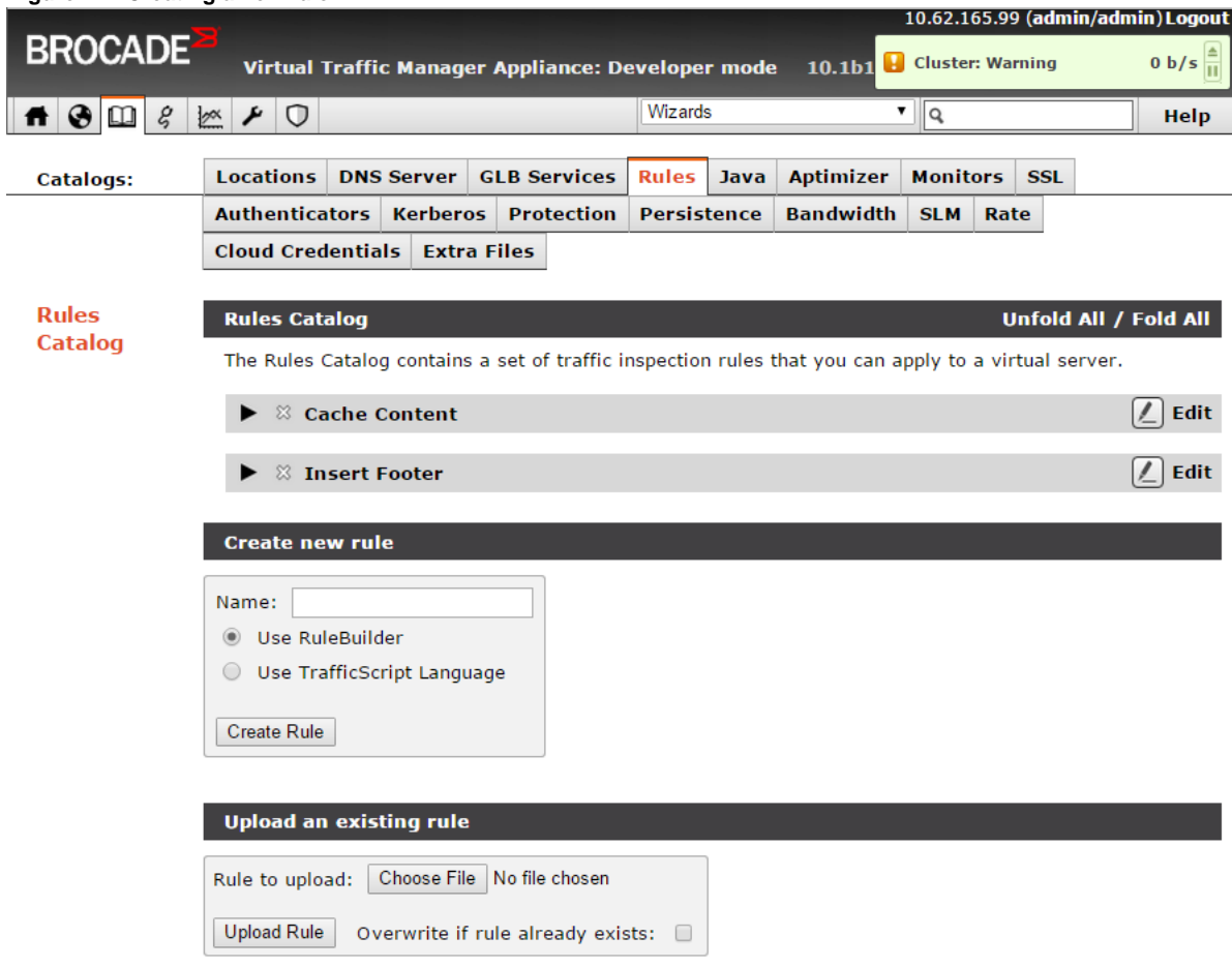
Figure 1-2. Creating a new rule
