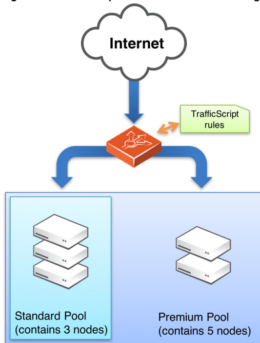
Figure 3-1. Customer prioritization scheme inserting cookies using TrafficScript
