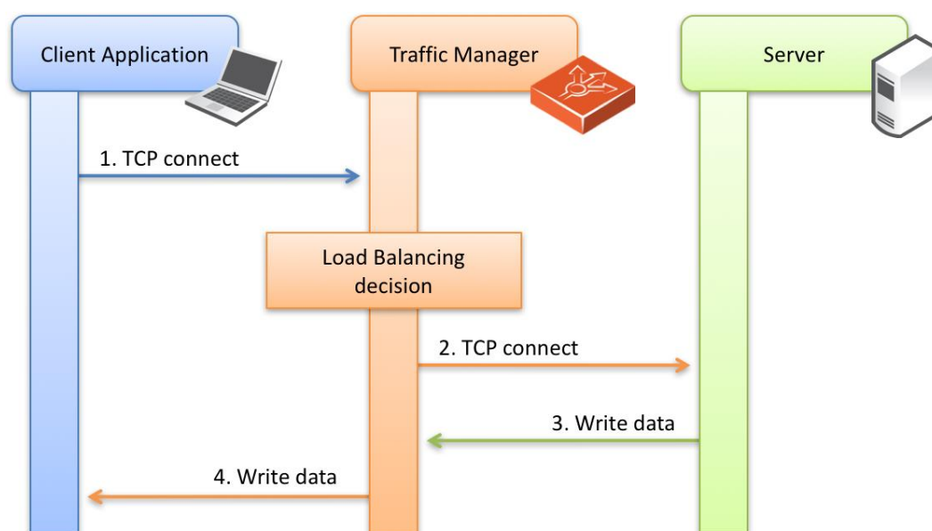
Fig 36. Server-first protocol load balancing
