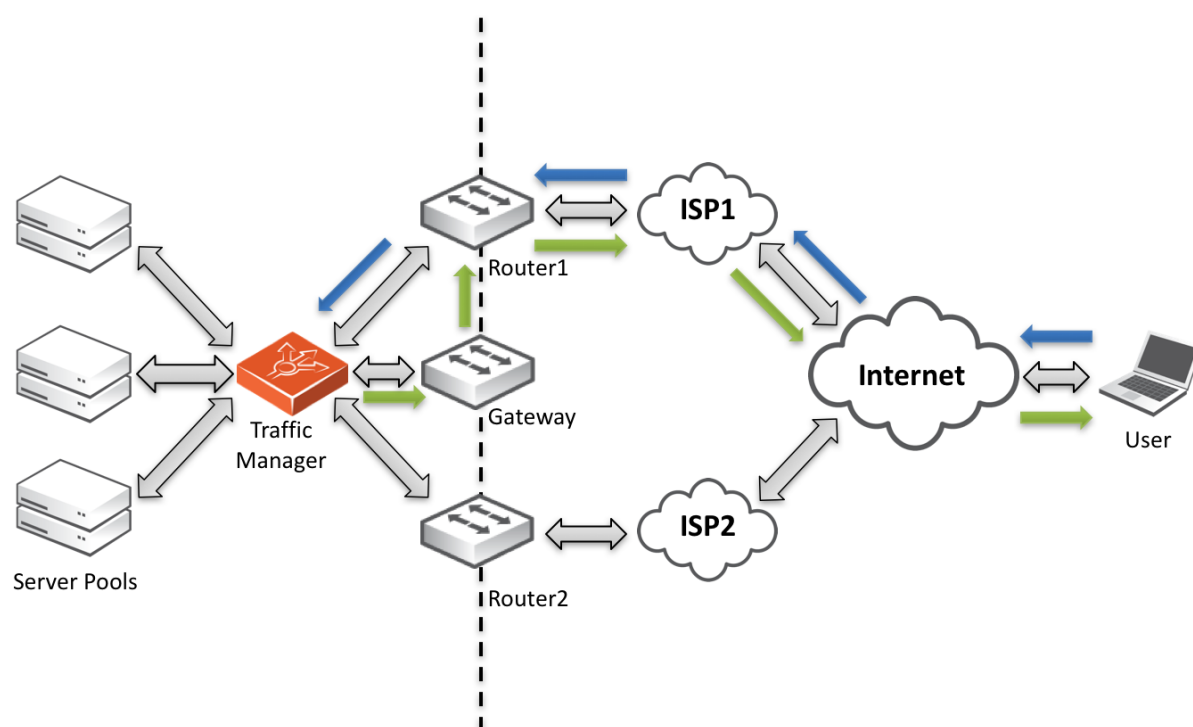
Fig 71. Employing a gateway router to perform connection tracking
