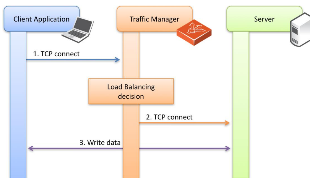
Fig 39. Load balancing with generic streaming protocols
