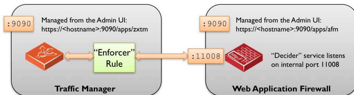
Fig 31. The Traffic Manager's Enforcer TrafficScript rule forwards requests to the default local port 11008 for inspection by the Decider service. The Decider returns a "Permit" or "Deny" decision and the Enforcer rule applies the decision.
