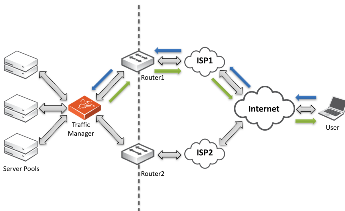
Fig 72. Return path routing is enabled
