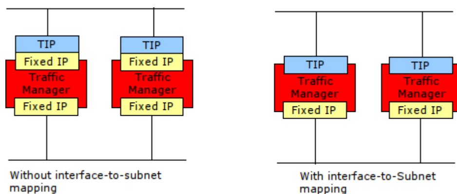
Fig 19. Interface to subnet mapping
