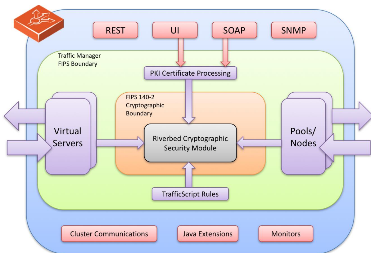
Fig 86. The Traffic Manager FIPS boundary
