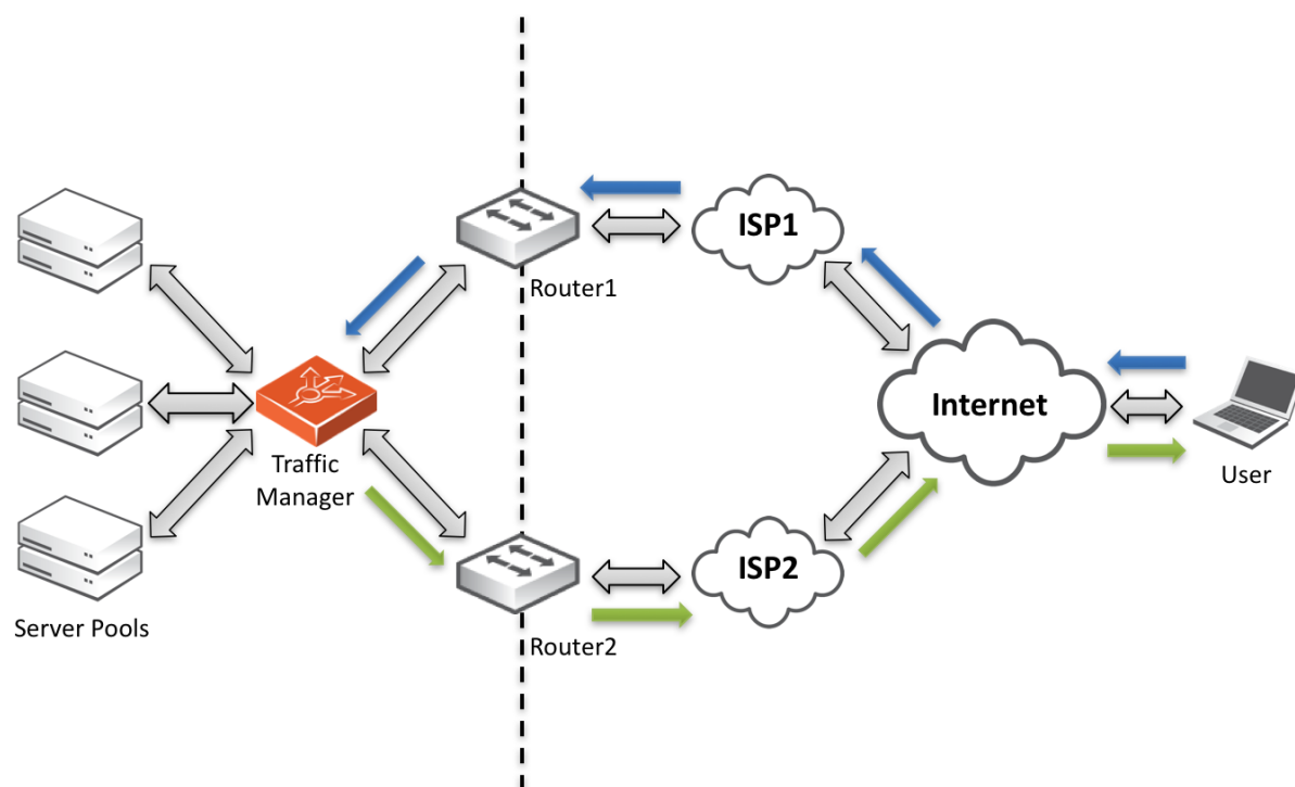
Fig 70. A typical lowest-cost route
