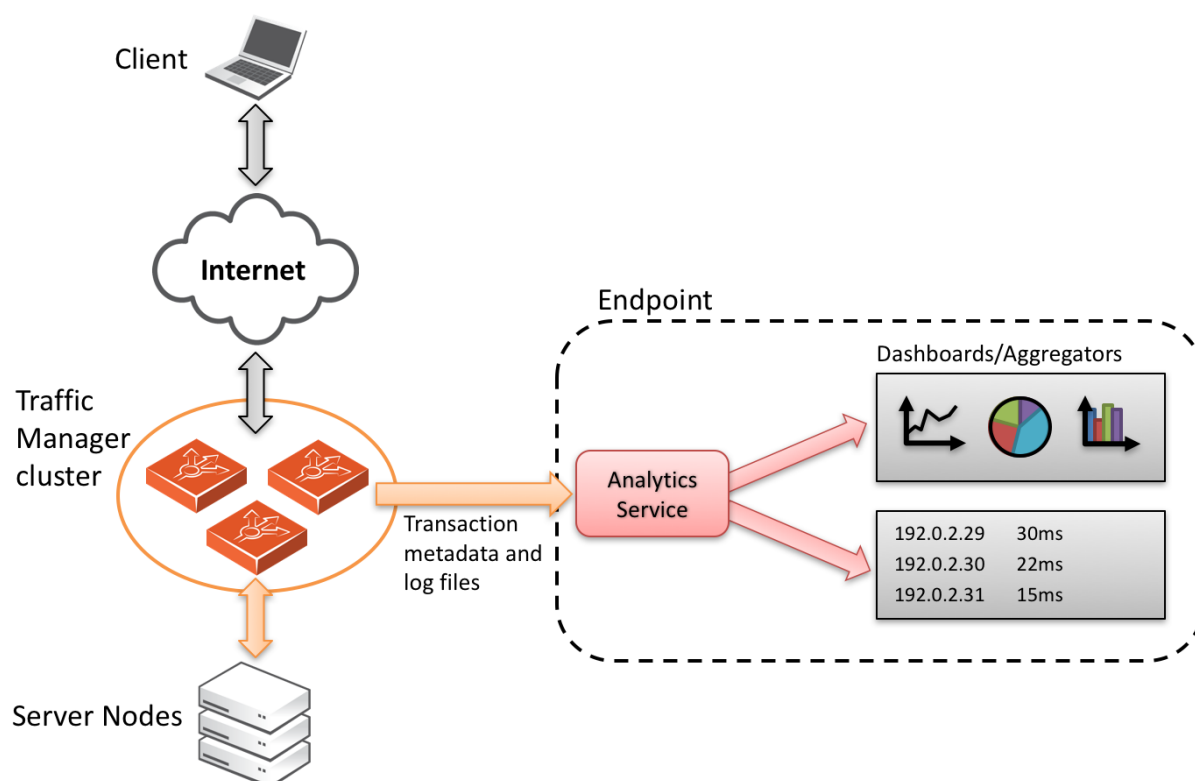
Fig 24. Streaming transaction metadata and log data to an external analytics endpoint
