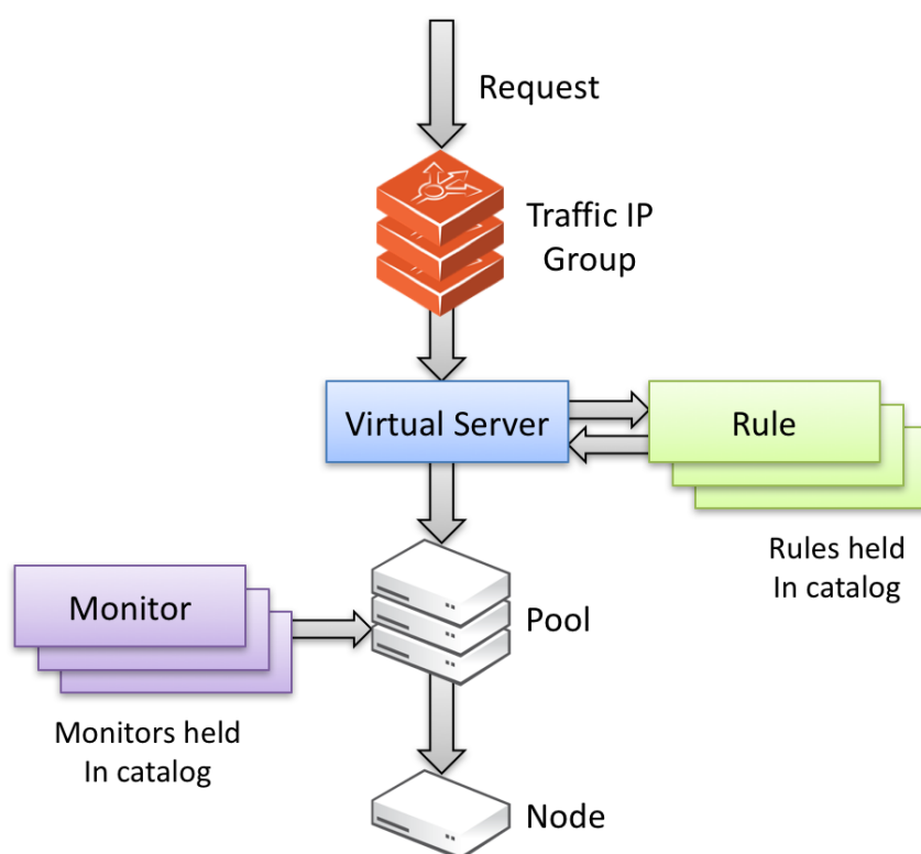
Fig 32. Analyzing, modifying and monitoring traffic using TrafficScript rules
