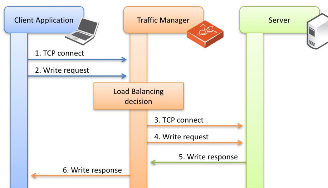
Fig 37. Client-first protocol load balancing
