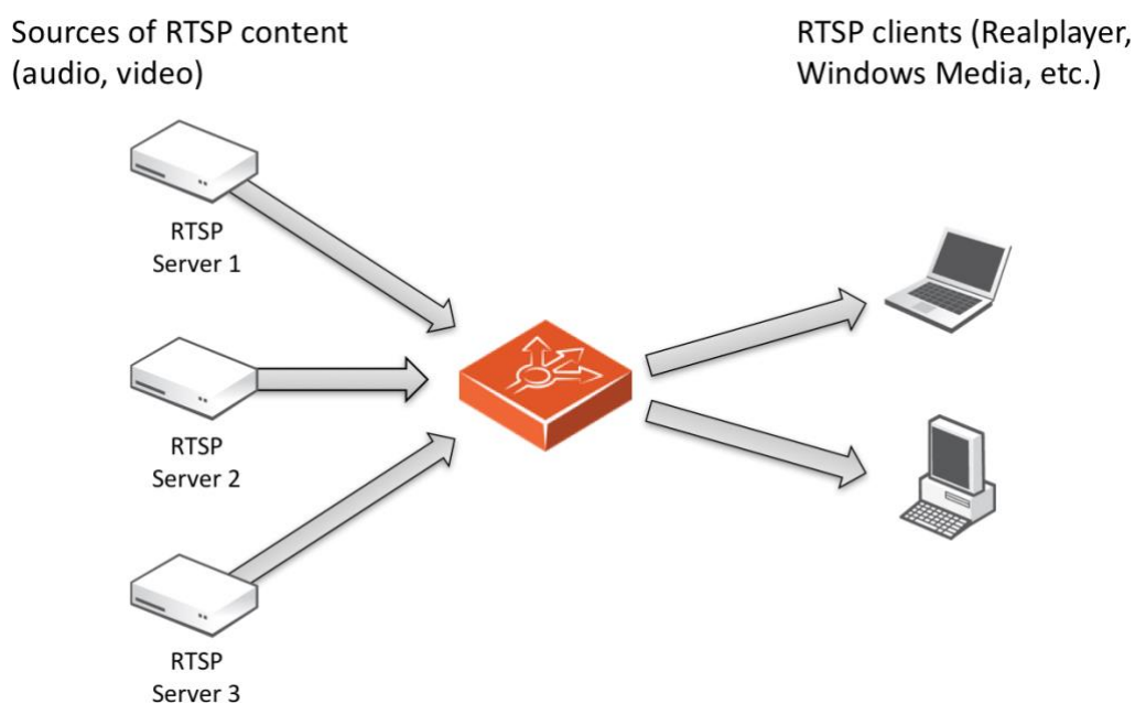
Fig 40. A Traffic Manager acting as a load balancer for standard RTSP content traffic
