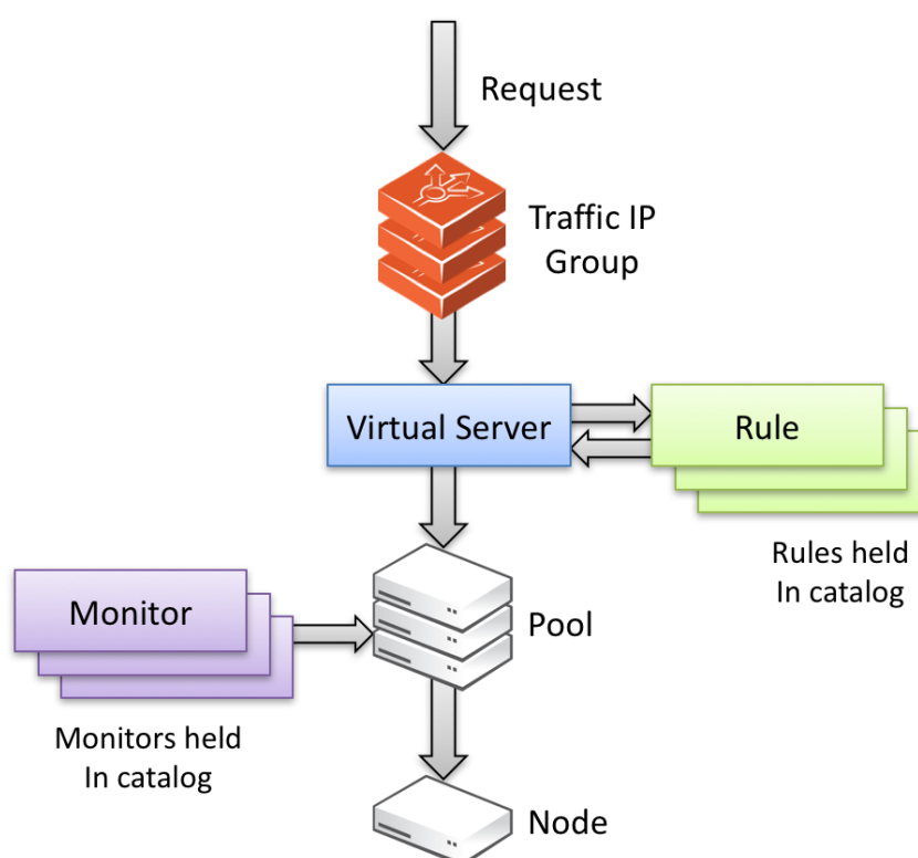
Fig 32. Analyzing, modifying and monitoring traffic using TrafficScript rules
