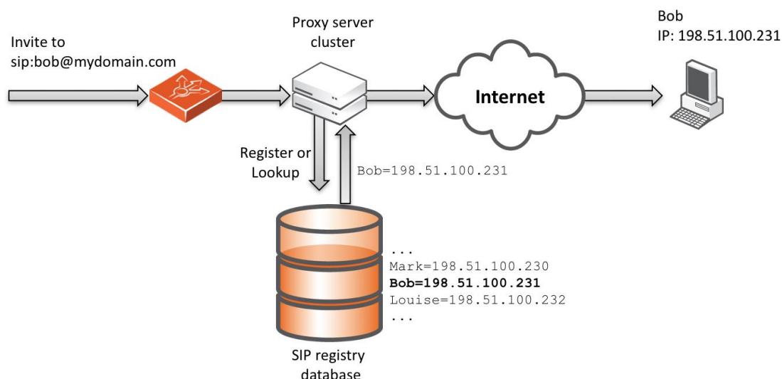
Fig 42. Detail of how an IP phone call using SIP would work with a Traffic Manager
