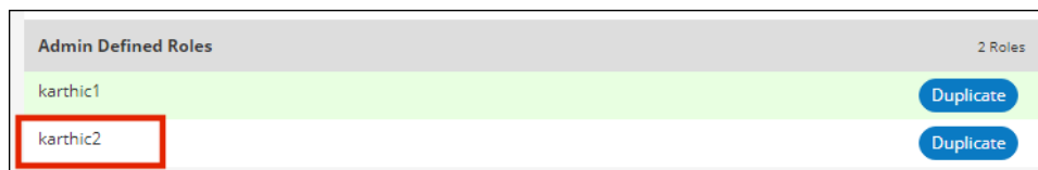
FIGURE 317 Duplicated Role
