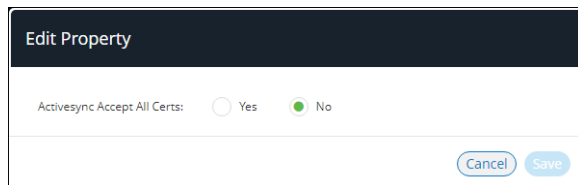
FIGURE 166 Edit Property
